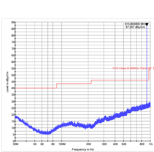
30MHz – 1GHz
