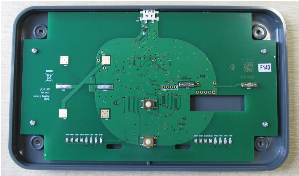
Figure 1: PCB top
