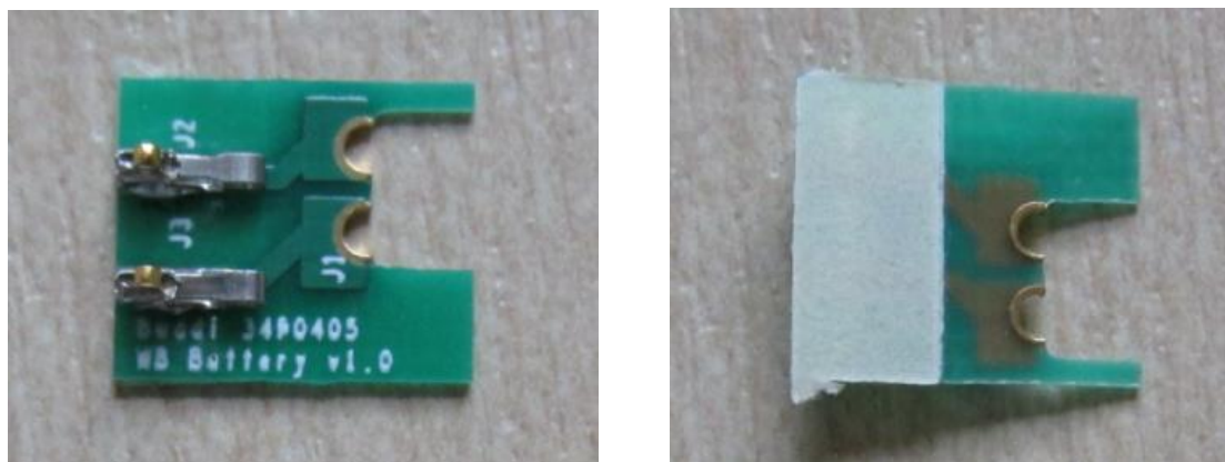
Figure 3: battery PCB, top and bottom
