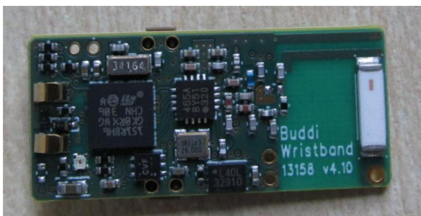
Figure 4: PCB top
