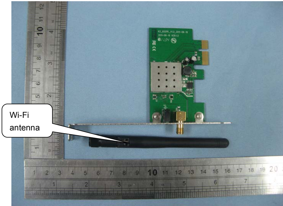
TOTAL VIEW OF EUT
