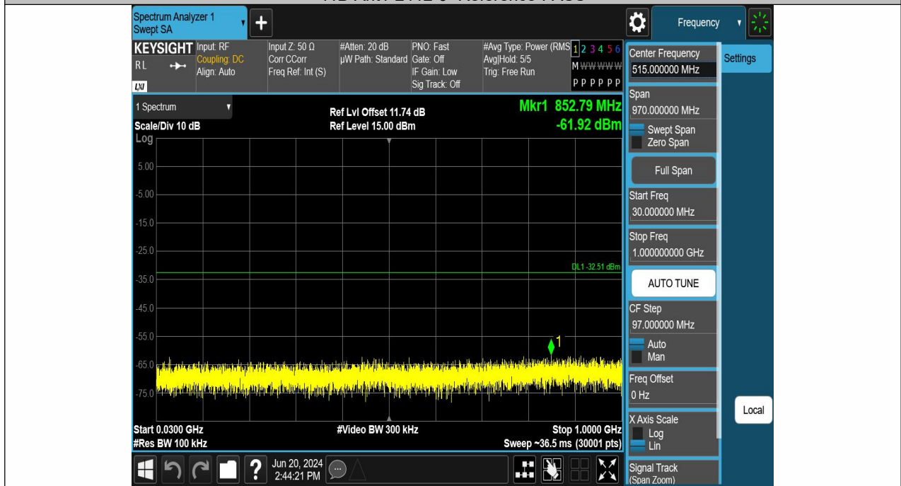
11B-Ant1-2412-30~1000-PASS
