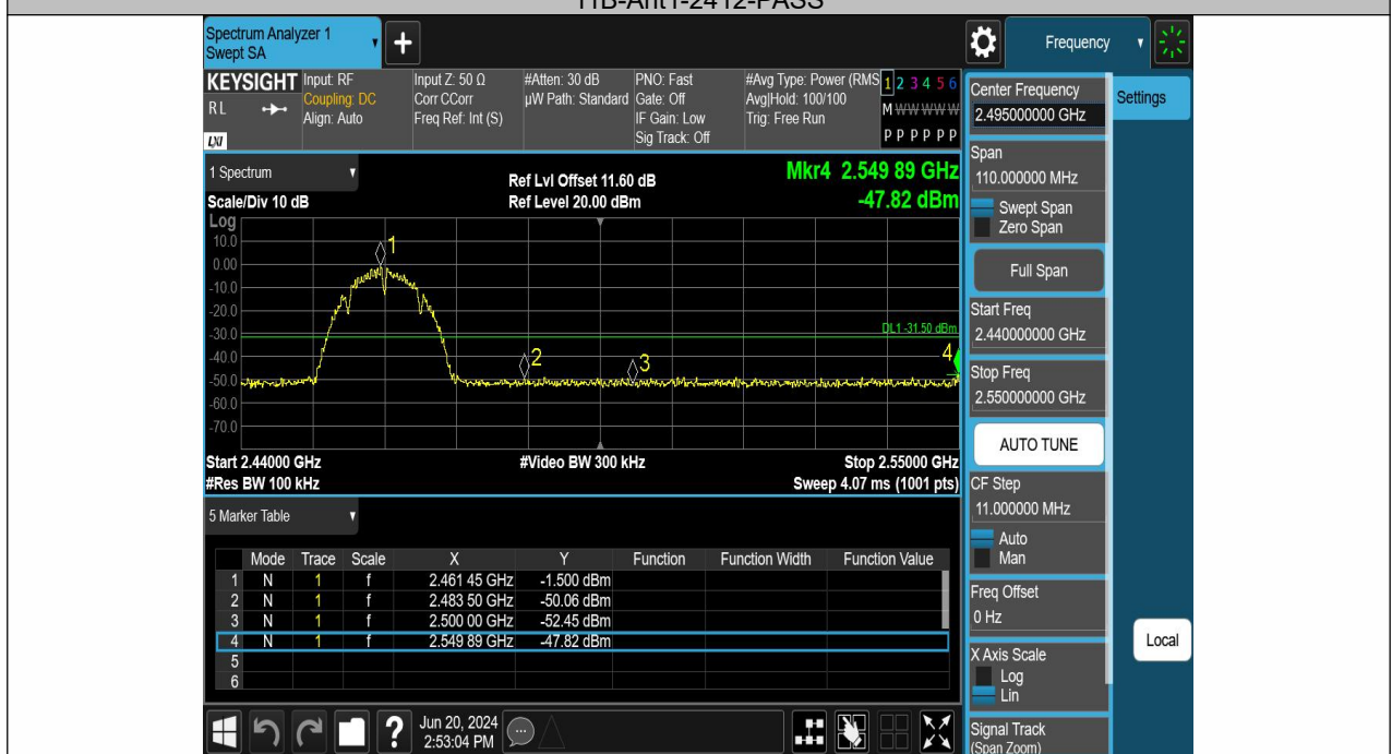
11B-Ant1-2462-PASS
