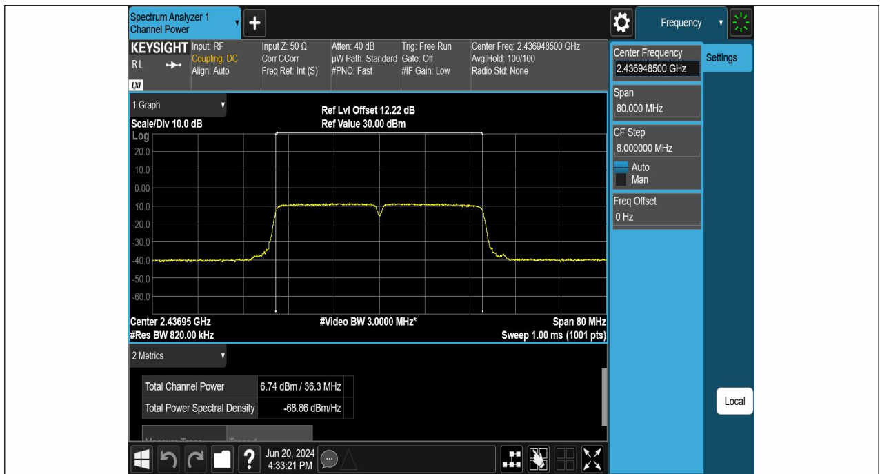
11N40SISO-Ant1-2437-PASS
