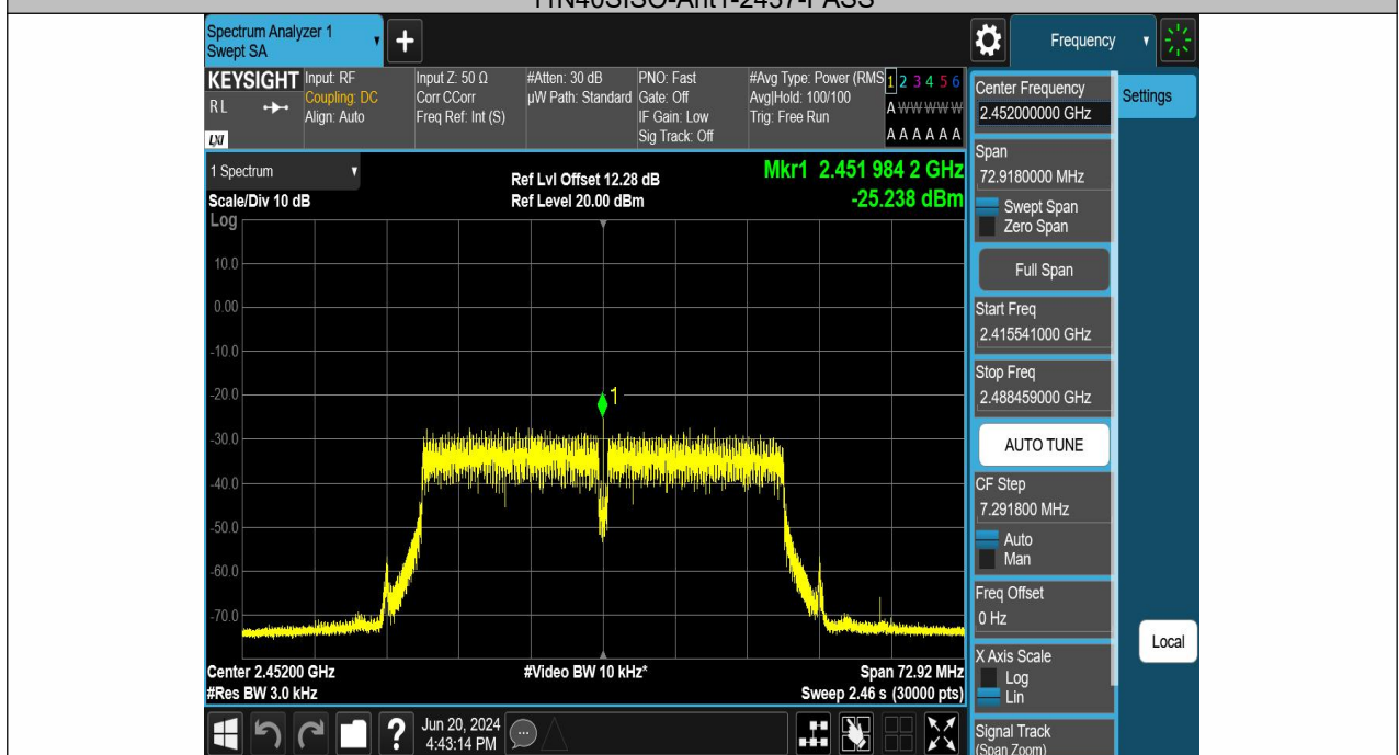
11N40SISO-Ant1-2452-PASS
