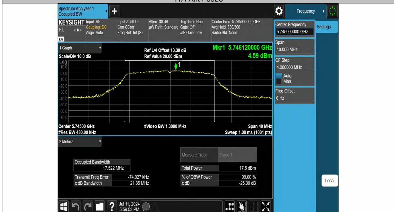
11N20SISO-Ant1-5745
