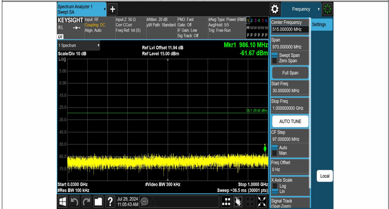
11N40SISO-Ant1-2437-30~1000-PASS
