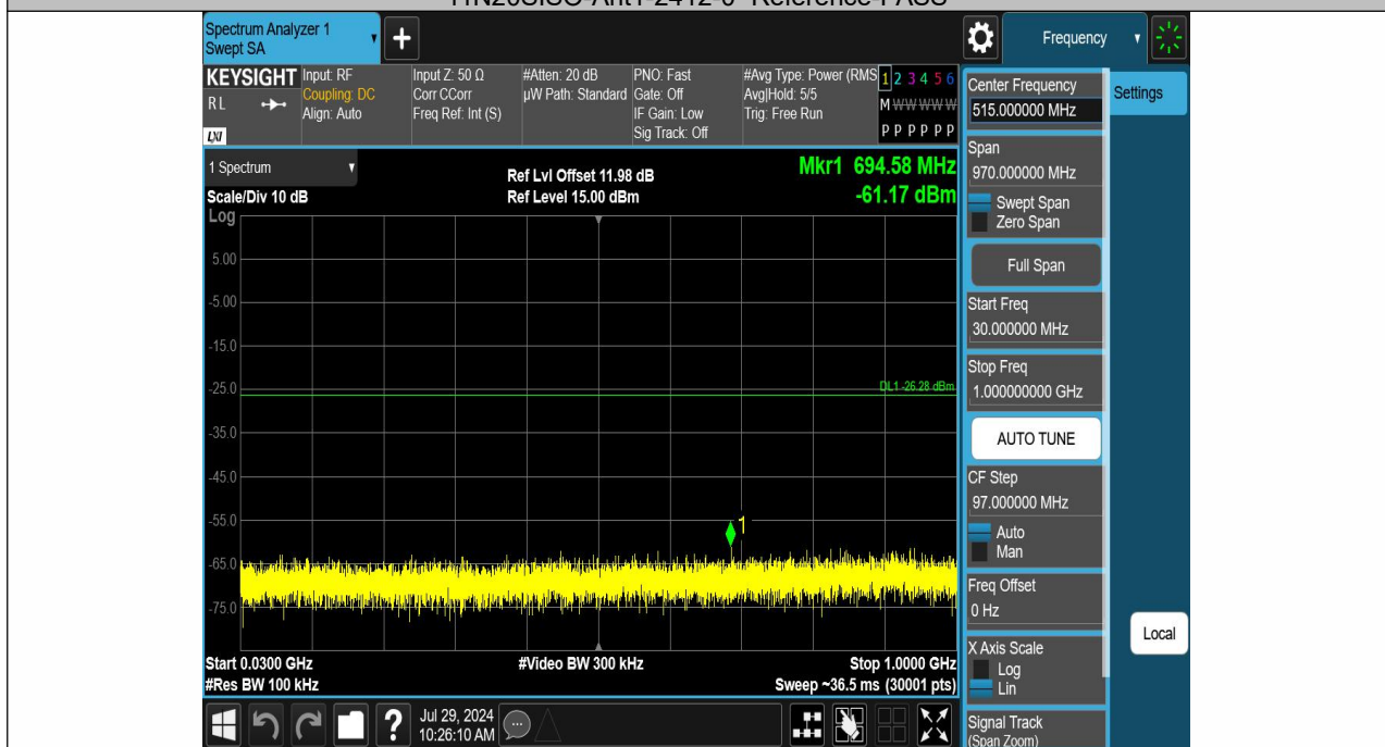
11N20SISO-Ant1-2412-30~1000-PASS
