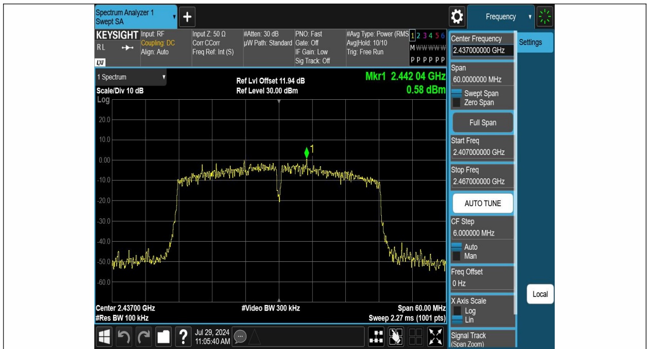
11N40SISO-Ant1-2437-0~Reference-PASS
