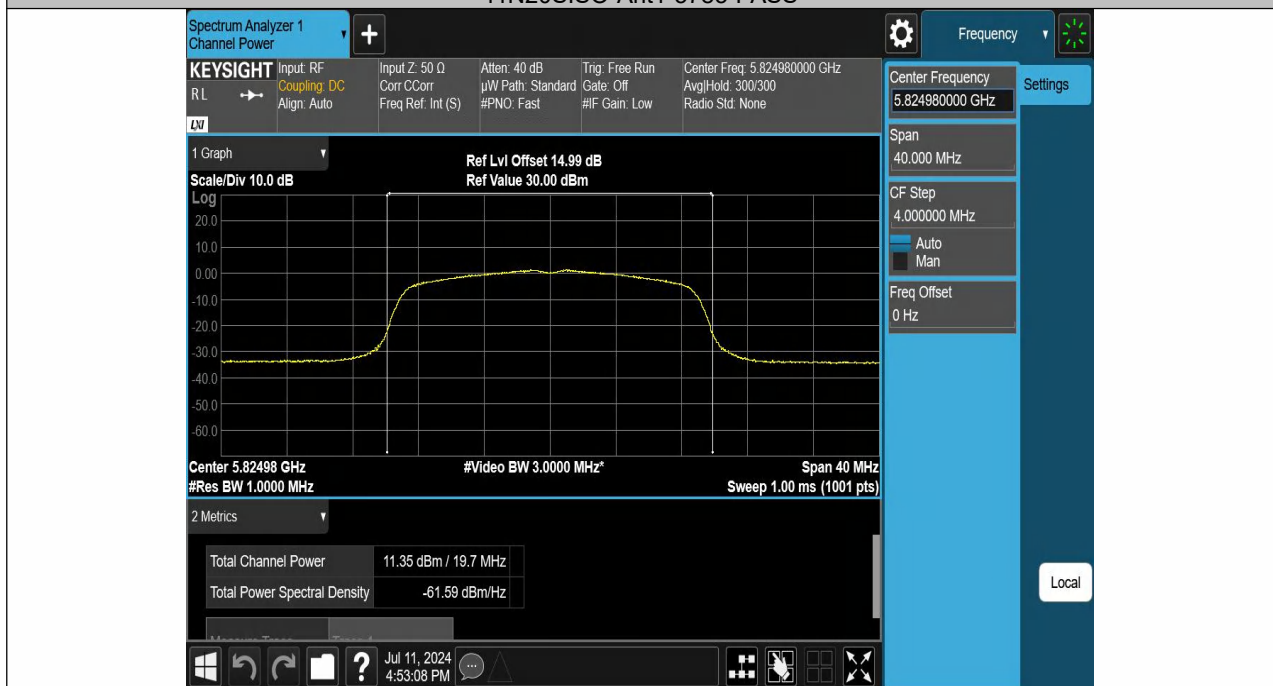
11N20SISO-Ant1-5825-PASS
