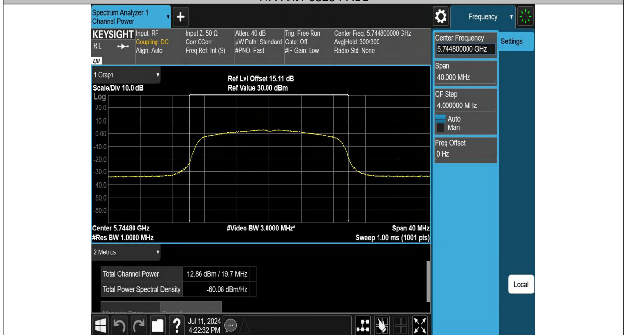
11N20SISO-Ant1-5745-PASS
