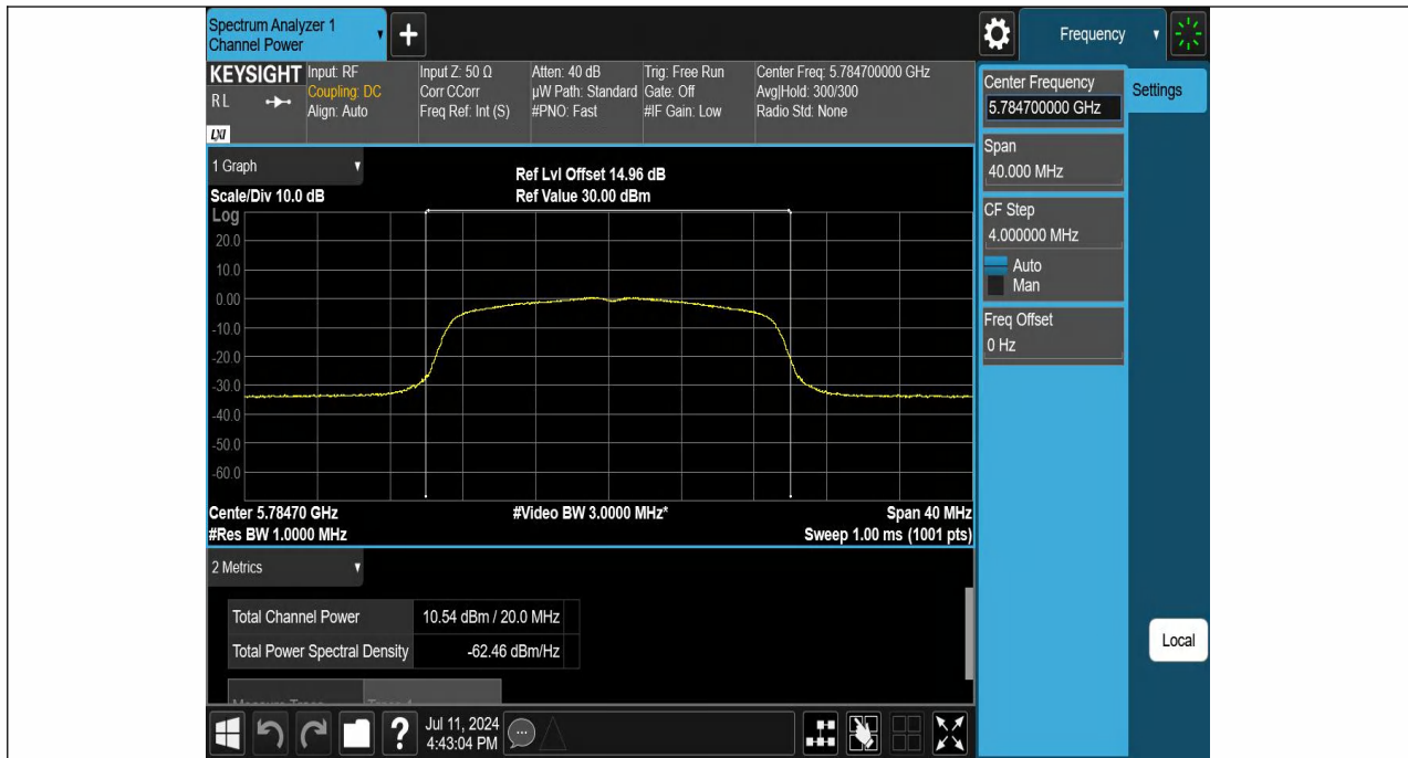
11N20SISO-Ant1-5785-PASS
