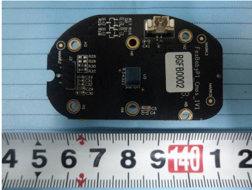
EUT –Image Sensor PCB Board Top View
