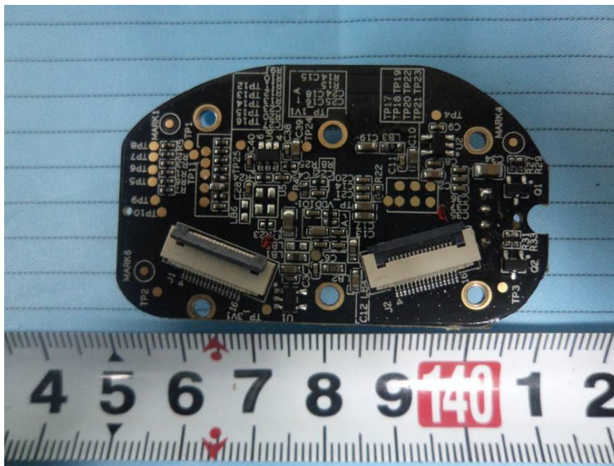
EUT –Image Sensor PCB Board Bottom View
