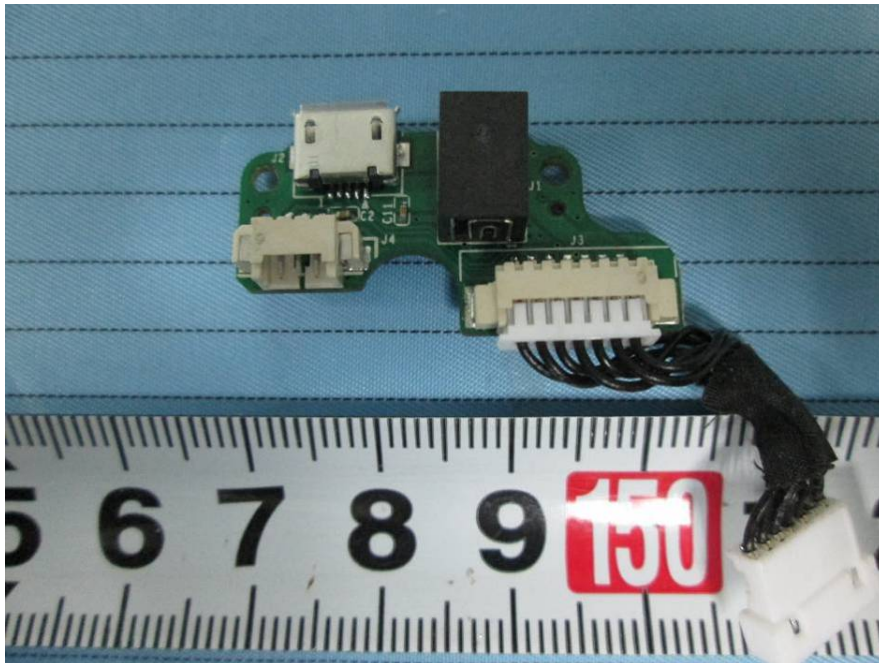
EUT –External Port PCB Board Top View
