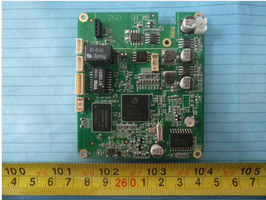
EUT –Main Board Without WiFi Module Board Top View
