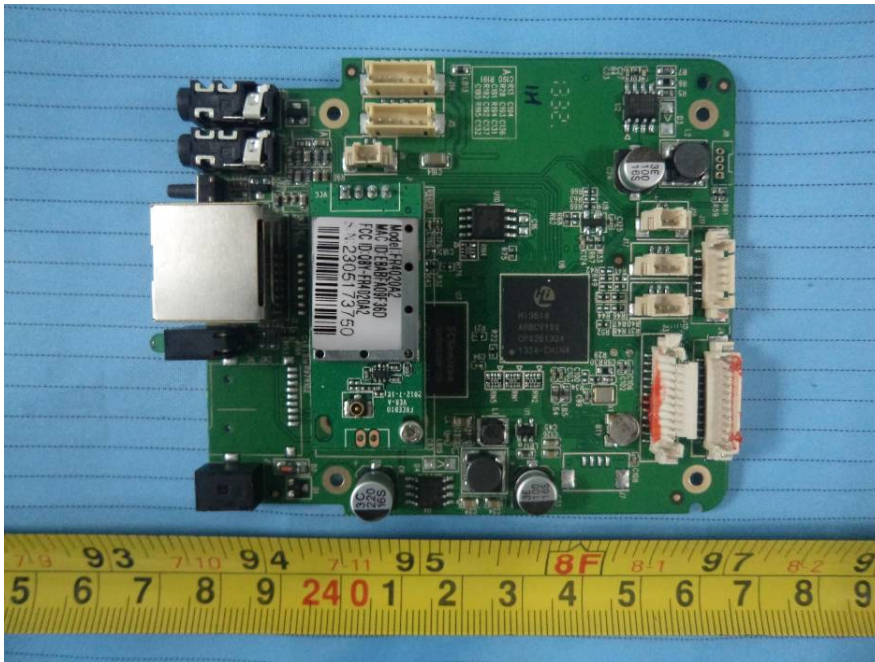
EUT – Main Board with WiFi Module Board Top View
