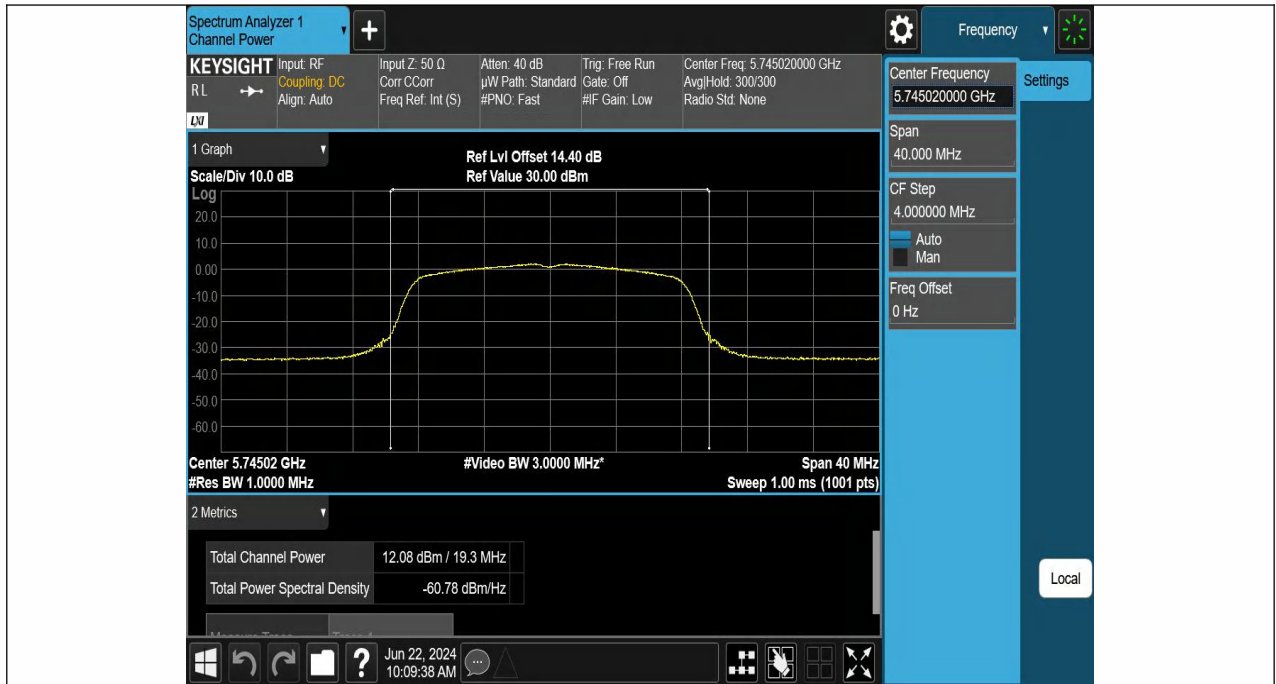
11A-Ant1-5745-PASS
