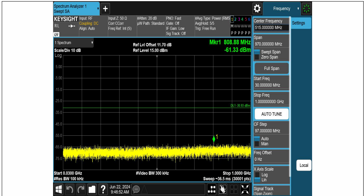
11N40SISO-Ant1-2422-30~1000-PASS
