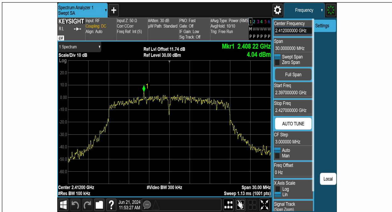
11N20SISO-Ant1-2412-0~Reference-PASS
