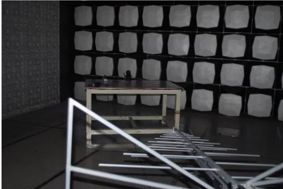
Radiated Spurious Emission Test Setup
