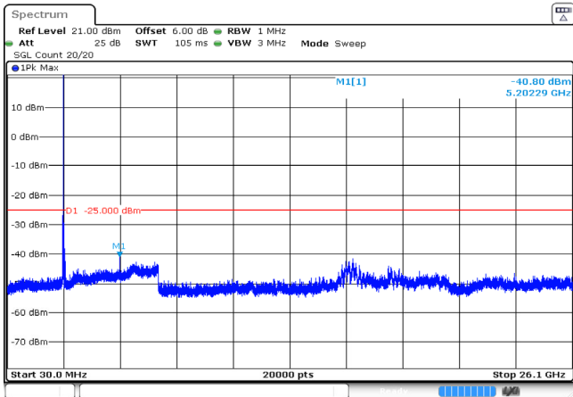
20MHz_High_QPSK_1@0 -40.80dBm
