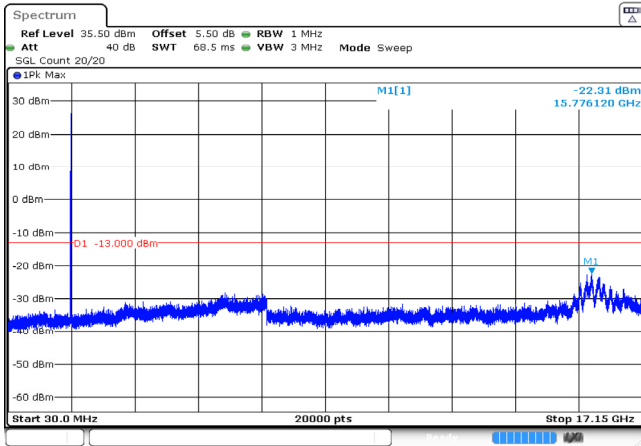
10MHz_Low_QPSK_1@0 -22.31dBm
