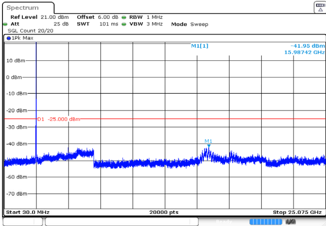
15MHz_Low_QPSK_1@0 -41.95dBm
