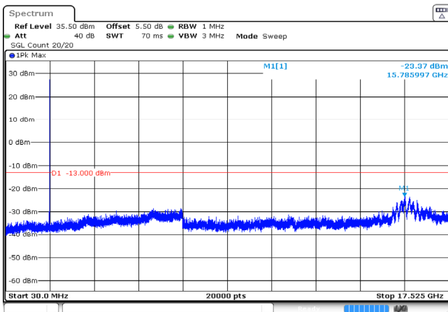
5MHz_High_QPSK_1@0 -23.37dBm
