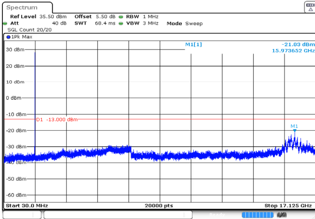
5MHz_Low_QPSK_1@0 -21.03dBm
