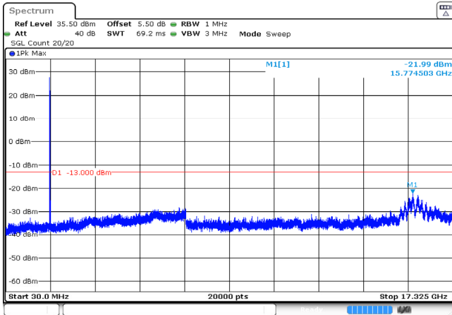
15MHz_Middle_QPSK_1@0 -21.99dBm
