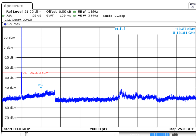
20MHz_High_QPSK_1@0 -40.57dBm
