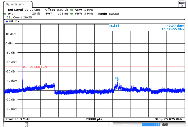
15MHz_Low_QPSK_75@0 -40.37dBm
