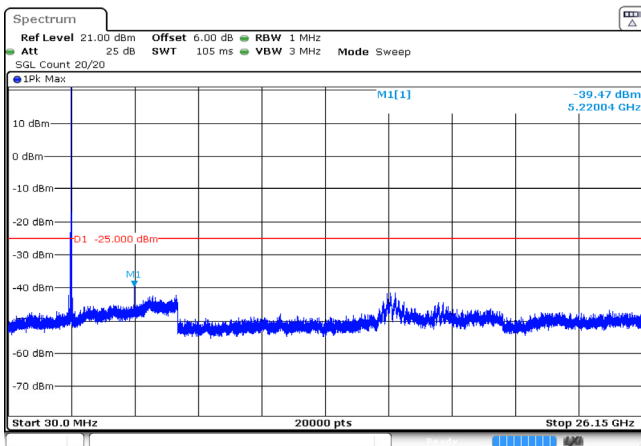
10MHz_High_QPSK_1@0 -39.47dBm
