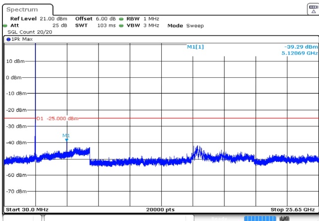
10MHz_High_QPSK_1@0 -39.29dBm
