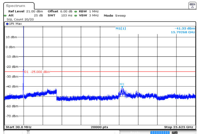
15MHz_High_QPSK_75@0 -41.33dBm
