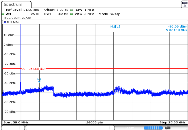
10MHz_Middle_QPSK_1@0 -39.98dBm
