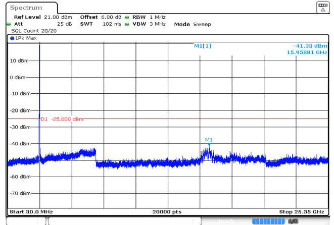
20MHz_Middle_QPSK_100@0 -41.33dBm
