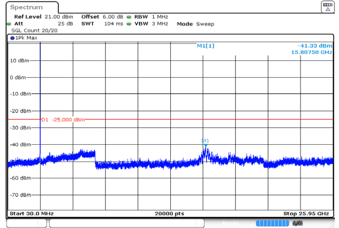
5MHz_Middle_QPSK_25@0 -41.33dBm
