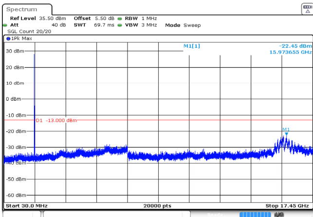
20MHz_High_QPSK_1@0 -22.45dBm
