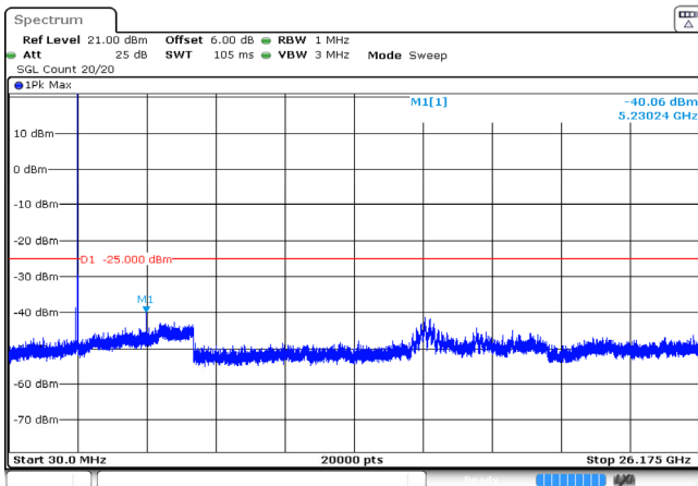
5MHz_High_QPSK_1@0 -40.06dBm
