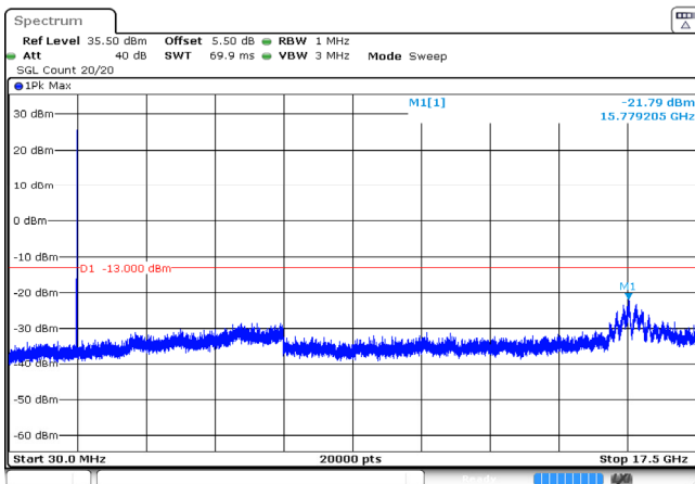
10MHz_High_QPSK_1@0 -21.79dBm
