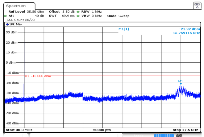
10MHz_High_QPSK_50@0 -21.92dBm
