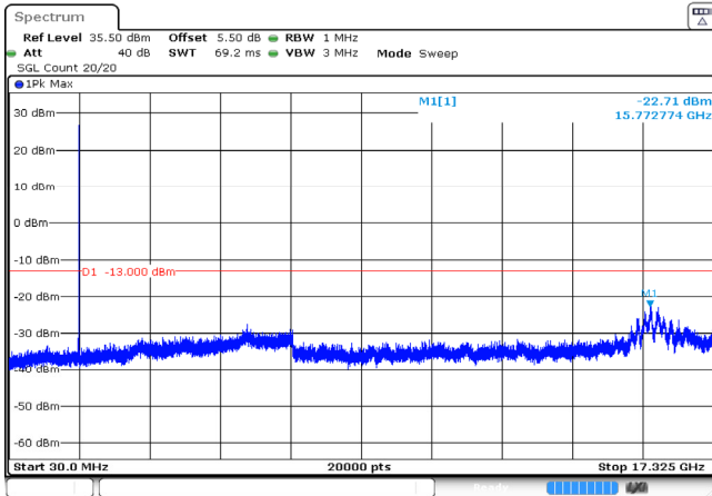
5MHz_Middle_QPSK_1@0 -22.71dBm
