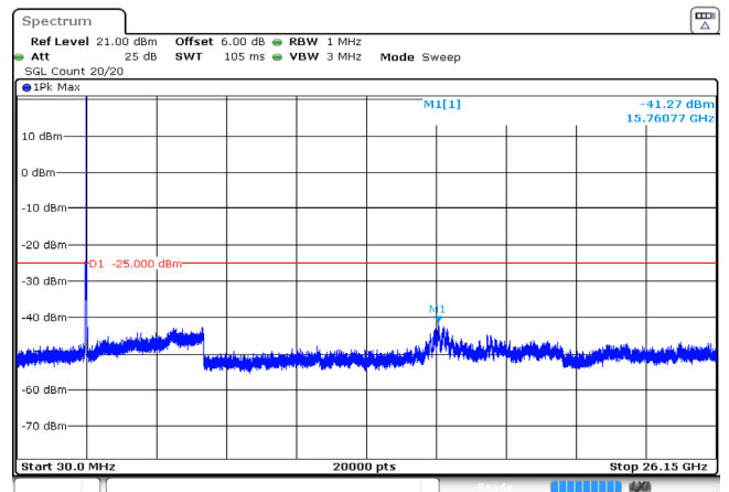
10MHz_High_QPSK_50@0 -41.27dBm
