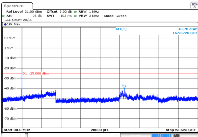
15MHz_High_QPSK_1@0 -40.78dBm
