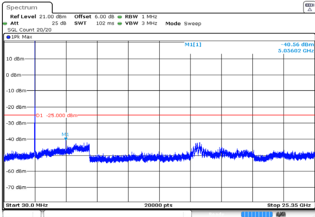
15MHz_Middle_QPSK_1@0 -40.56dBm
