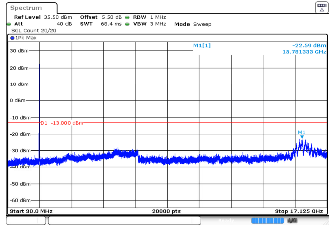
5MHz_Low_QPSK_25@0 -22.59dBm
