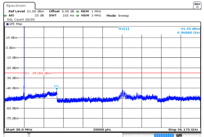
5MHz_High_QPSK_25@0 -41.43dBm
