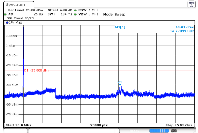
20MHz_Middle_QPSK_100@0 -40.81dBm
