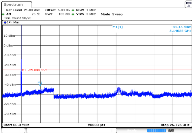
15MHz_Low_QPSK_1@0 -41.45dBm
