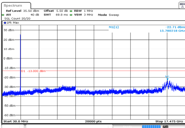
15MHz_High_QPSK_1@0 -22.71dBm
