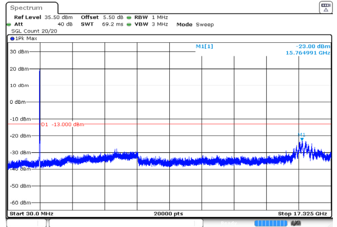
15MHz_Middle_QPSK_75@0 -23.00dBm
