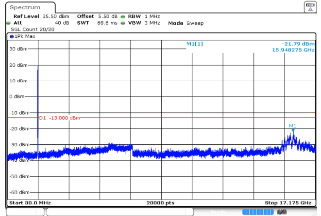
15MHz_Low_QPSK_75@0 -21.79dBm
