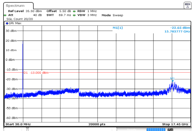
20MHz_High_QPSK_100@0 -22.65dBm
