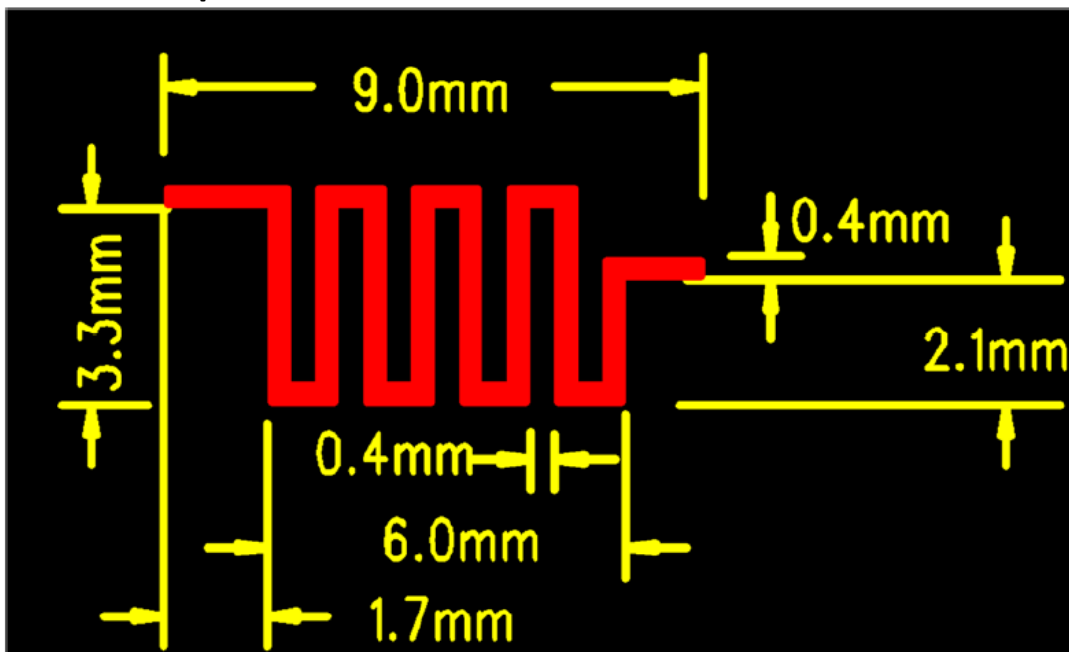
Antenna shape
