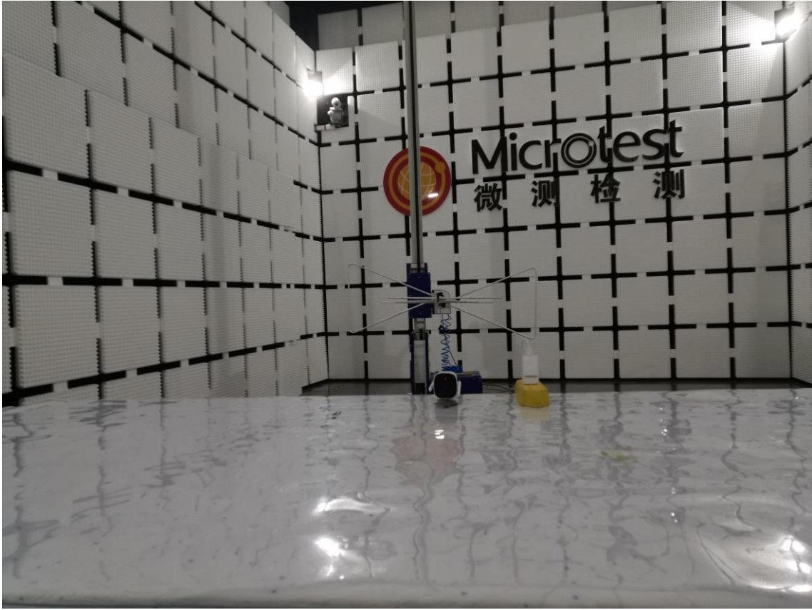
Radiated emission
