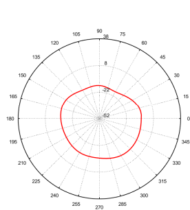
Total_Polar_E1_2.5GHz
