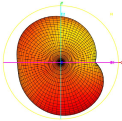
Total_3D_H_2.45GHz
