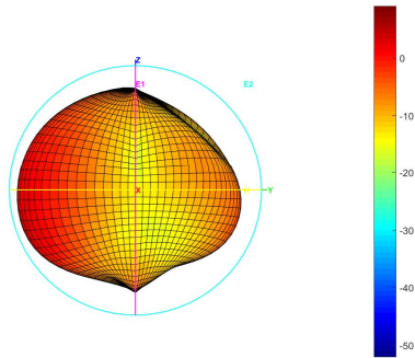
Total_3D_E2_2.5GHz
