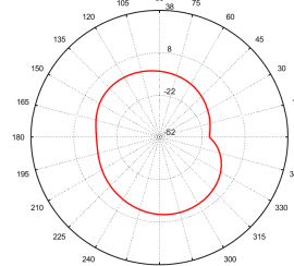
Total_Polar_H_2.45GHz
