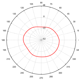
Total_Polar_E1_2.45GHz
