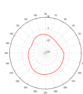
Total_Polar_E2_2.5GHz
