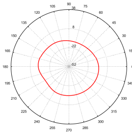
Total_Polar_E1_2.4GHz
