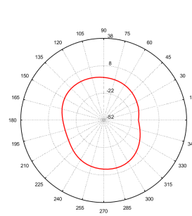
Total_Polar_H_2.5GHz
