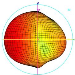
Total_3D_E2_2.45GHz
