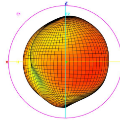
Total_3D_E1_2.45GHz
