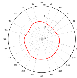
Total_Polar_E2_2.45GHz
