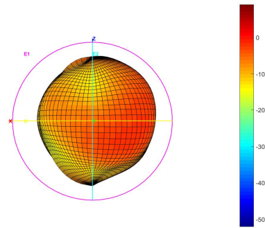
Total_3D_E1_2.5GHz
