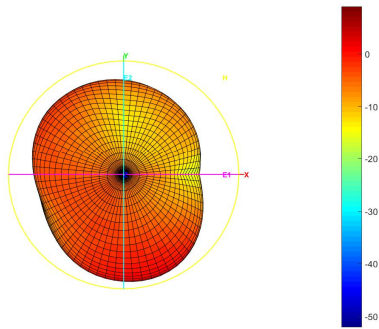
Total_3D_H_2.5GHz
