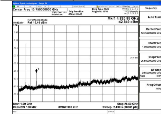
802.11g on Channel 01
