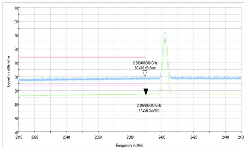
Fig.1. Frequency Band Edges: GFSK, 2402 MHz, 2.31 GHz – 2.45GHz
