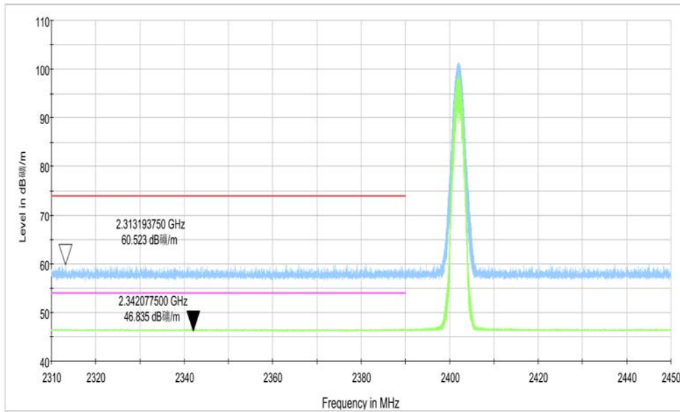
Fig.11. Frequency Band Edges: 8DPSK, Channel 0, 2.31 GHz - 2.45GHz
