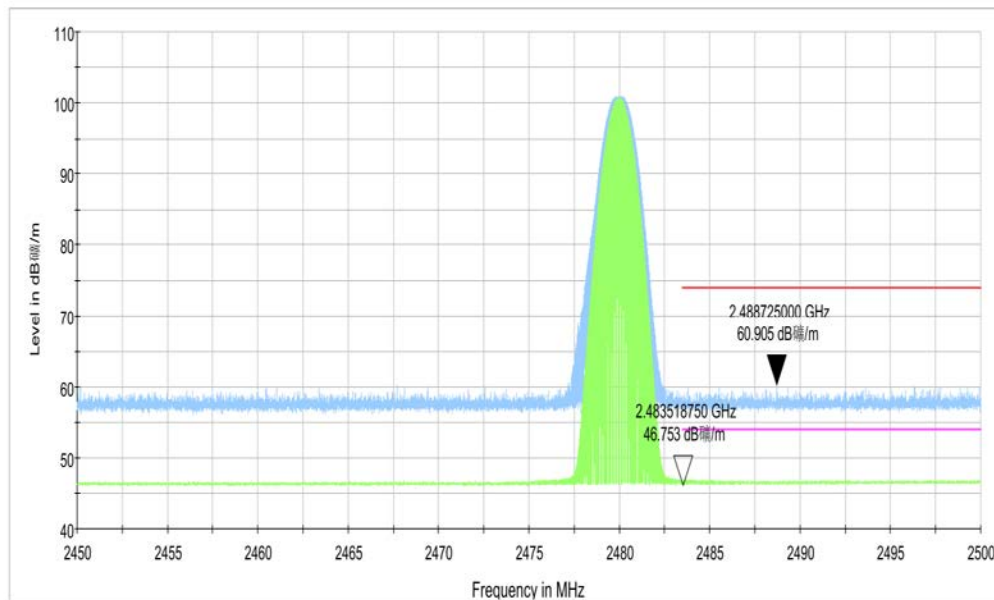
Fig.8. Frequency Band Edges: GFSK, Channel 78, Hopping Off, 2.45 GHz - 2.50GHz
