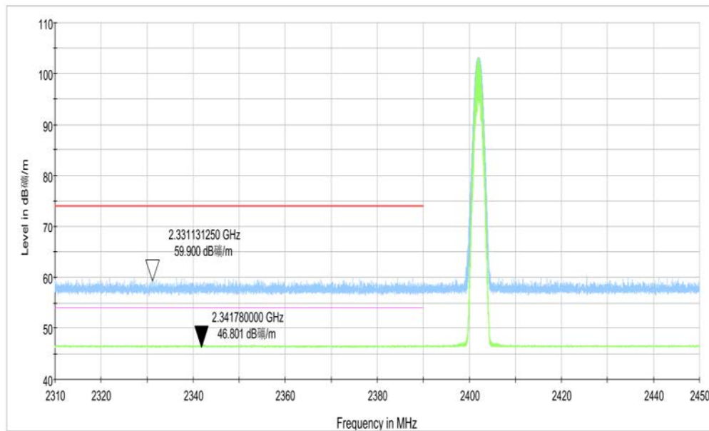
Fig.7. Frequency Band Edges: GFSK, Channel 0, Hopping Off, 2.31 GHz – 2.45GHz
