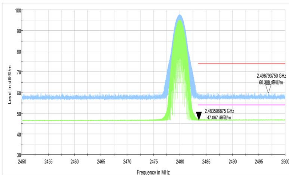
Fig.12. Frequency Band Edges: 8DPSK, Channel 78, 2.45 GHz - 2.50GHz
