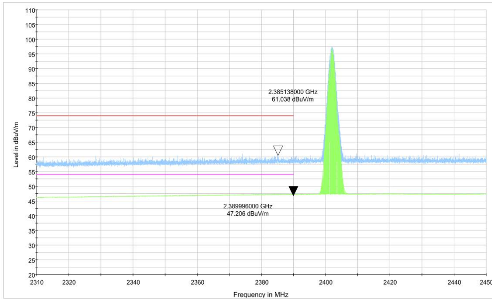
Fig.1. Frequency Band Edges: GFSK, Channel 0, 2.31 GHz – 2.45GHz
