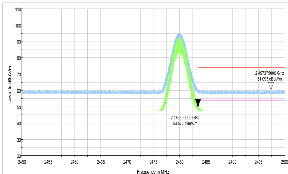
Fig.6. Frequency Band Edges: 8DPSK, Channel 78, 2.45 GHz - 2.50GHz
