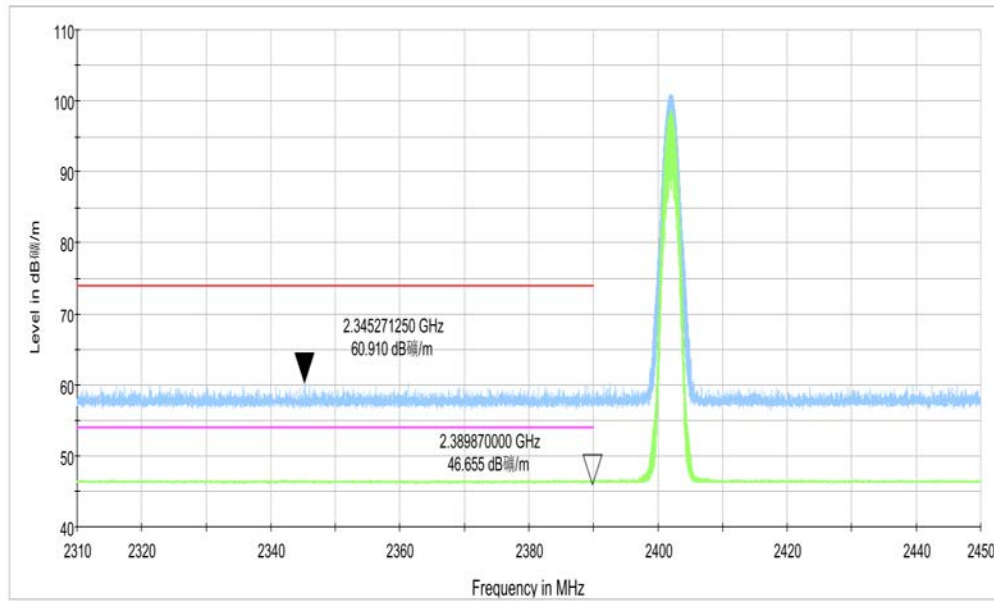
Fig.9. Frequency Band Edges: \pi/4 DQPSK, Channel 0, Hopping Off, 2.31 GHz - 2.45GHz
