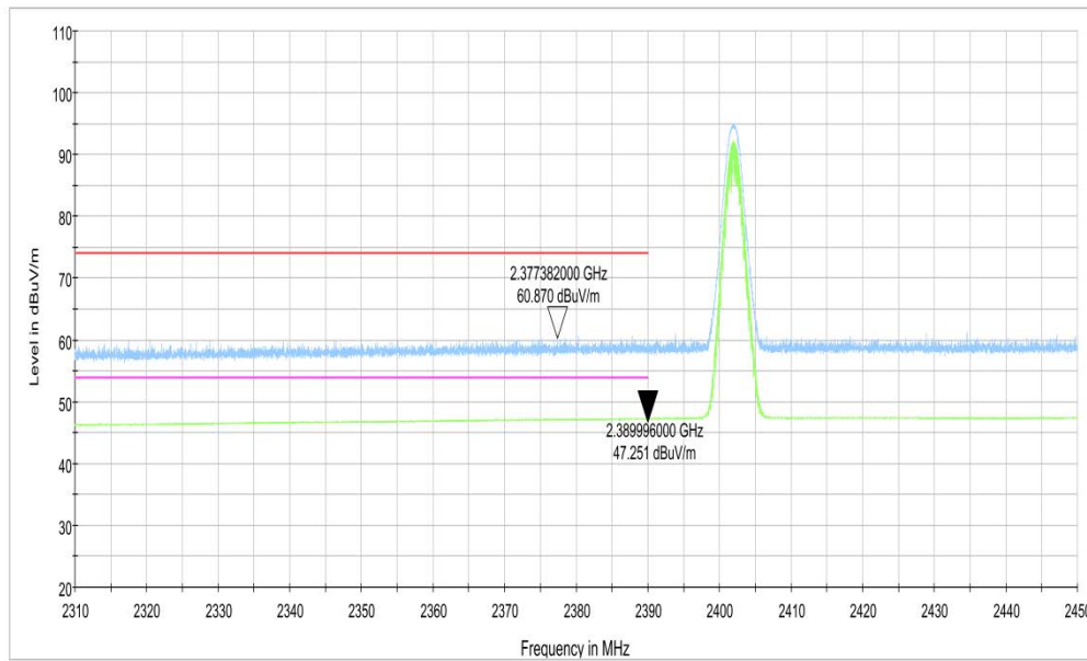
Fig.5. Frequency Band Edges: 8DPSK, Channel 0, 2.31 GHz - 2.45GHz
