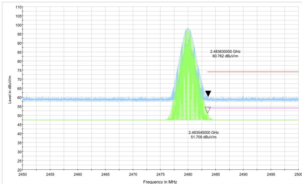
Fig.2. Frequency Band Edges: GFSK, Channel 78, 2.45 GHz - 2.50GHz
