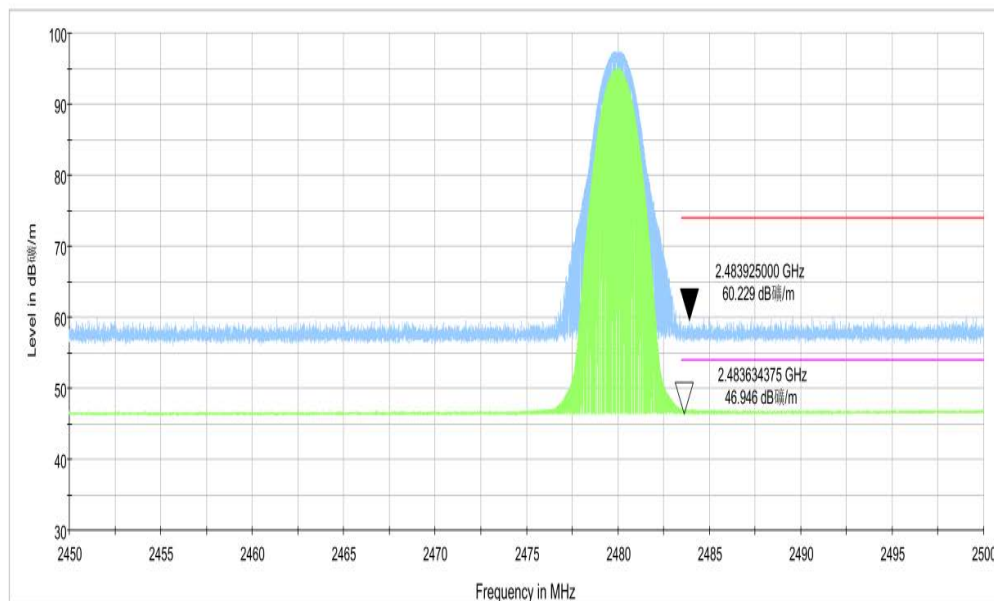
Fig.10. Frequency Band Edges: \pi/4 DQPSK, Channel 78, Hopping Off, 2.45 GHz - 2.50GHz
