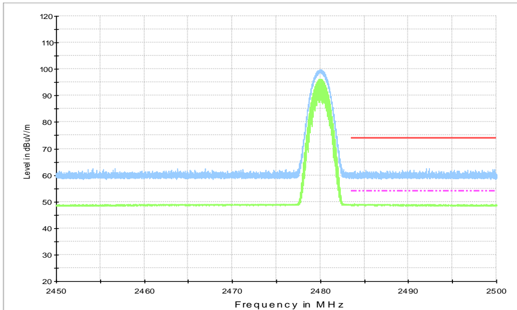
Fig.27. Frequency Band Edges: 8DPSK, Channel 78, 2.45 GHz - 2.50GHz
