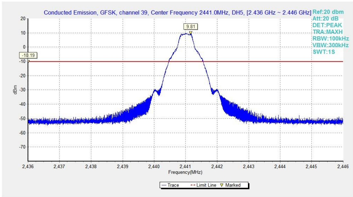
Fig.33. Conducted spurious emission: GFSK, Channel 39, 2441MHz
