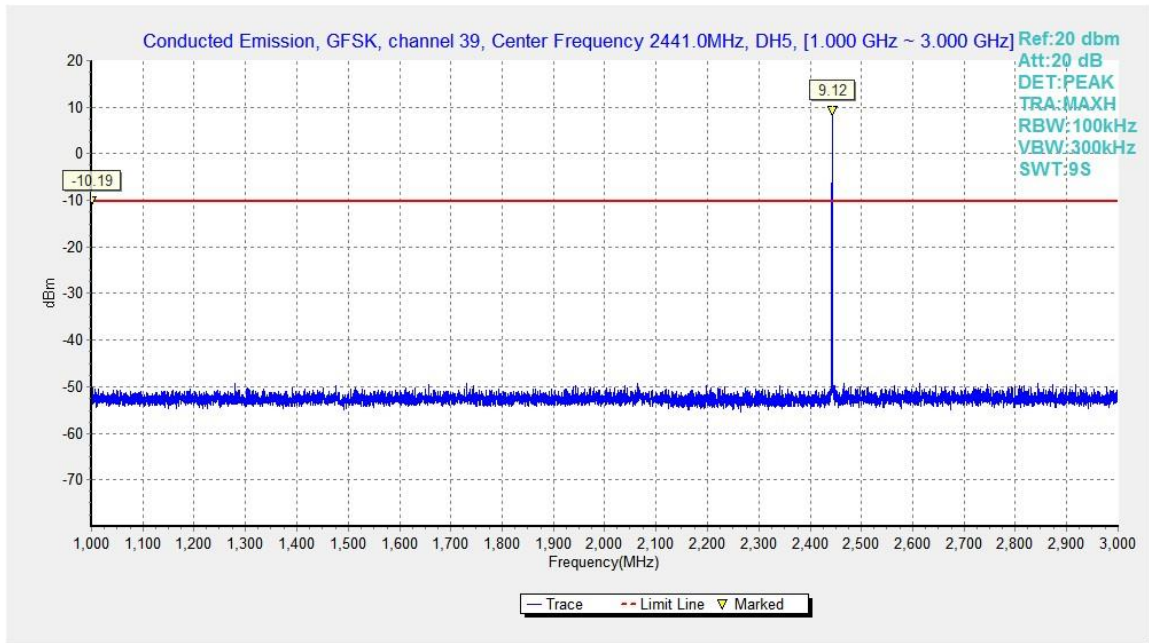
Fig.35. Conducted spurious emission: GFSK, Channel 39, 1GHz – 3GHz
