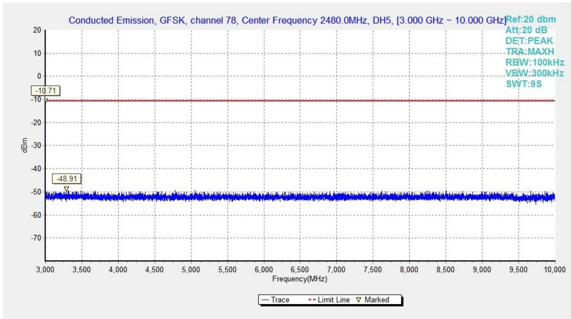
Fig.41. Conducted spurious emission: GFSK, Channel 78, 3GHz - 10GHz
