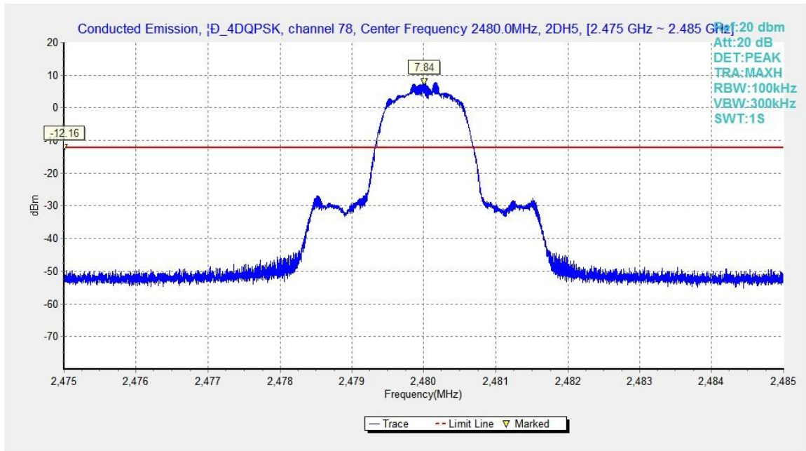
Fig.53. Conducted spurious emission: \pi/4 DQPSK, Channel 78, 2480MHz
