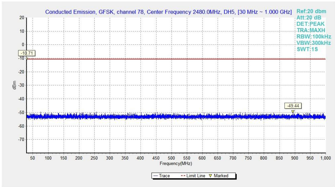
Fig.39. Conducted spurious emission: GFSK, Channel 78, 30MHz - 1GHz
