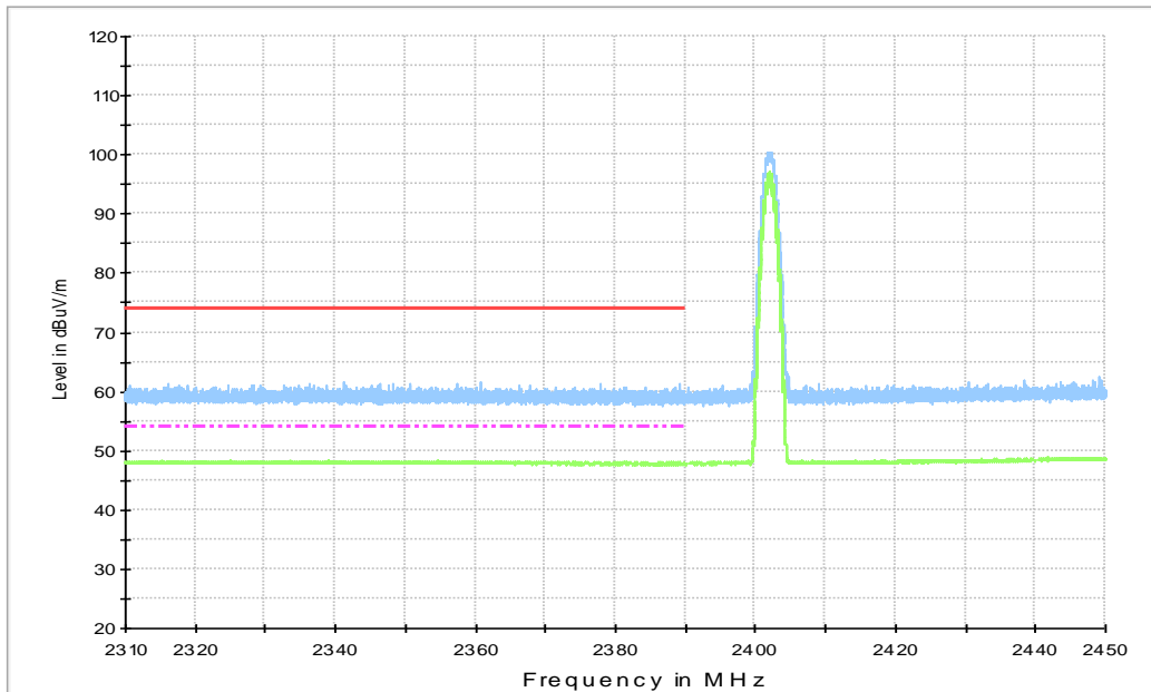
Fig.24. Frequency Band Edges: \pi/4 DQPSK, Channel 0, 2.31 GHz - 2.45GHz
