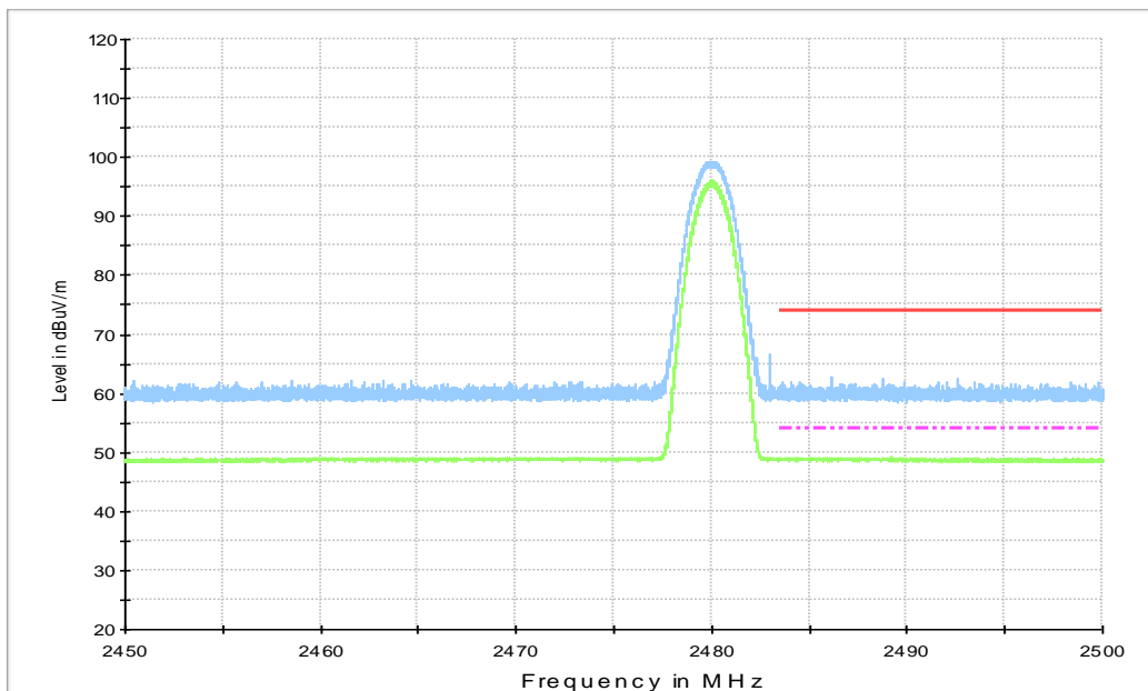
Fig.25. Frequency Band Edges: \pi/4 DQPSK, Channel 78, 2.45 GHz - 2.50GHz
