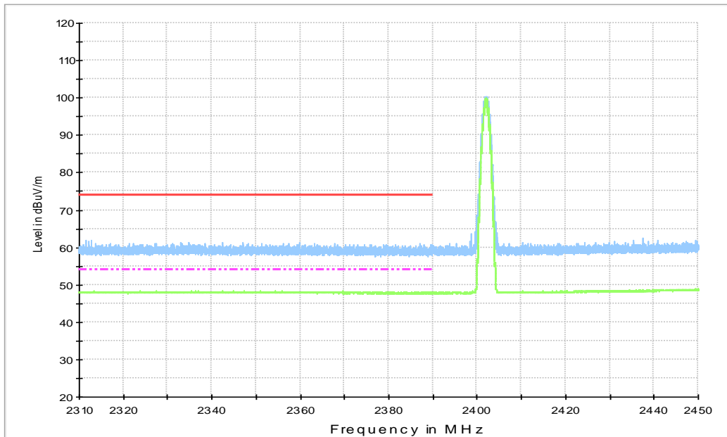
Fig.22. Frequency Band Edges: GFSK, Channel 0, 2.31 GHz – 2.45GHz
