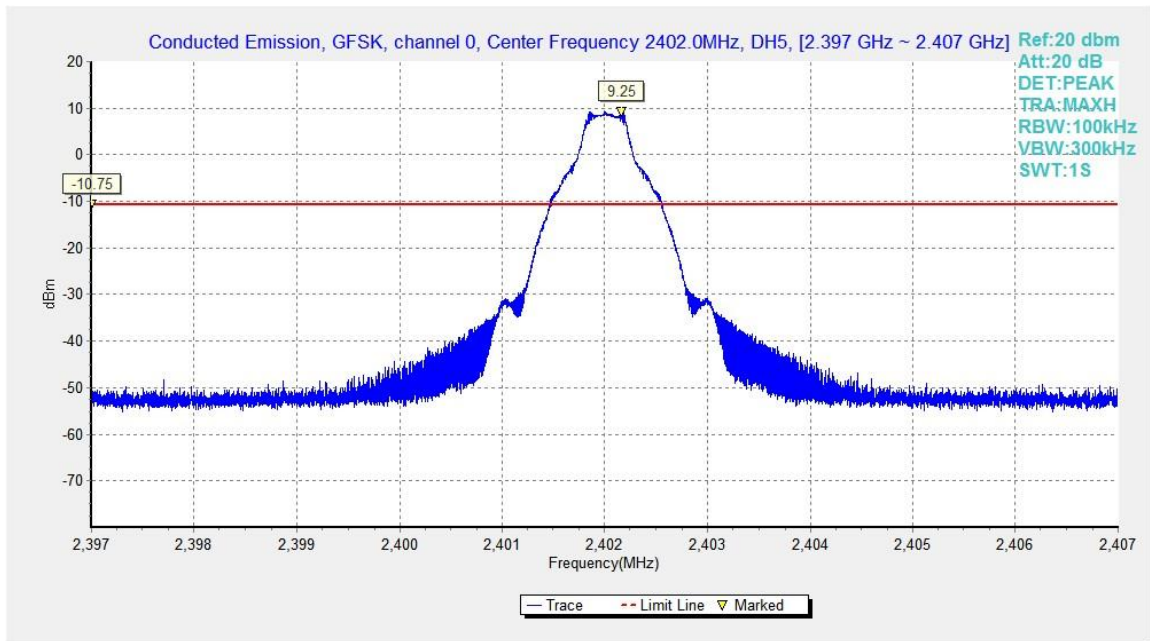
Fig.28. Conducted spurious emission: GFSK, Channel 0,2402MHz
