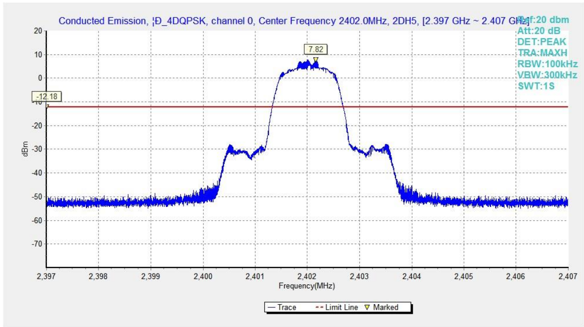
Fig.43. Conducted spurious emission: \pi/4 DQPSK, Channel 0, 2402MHz
