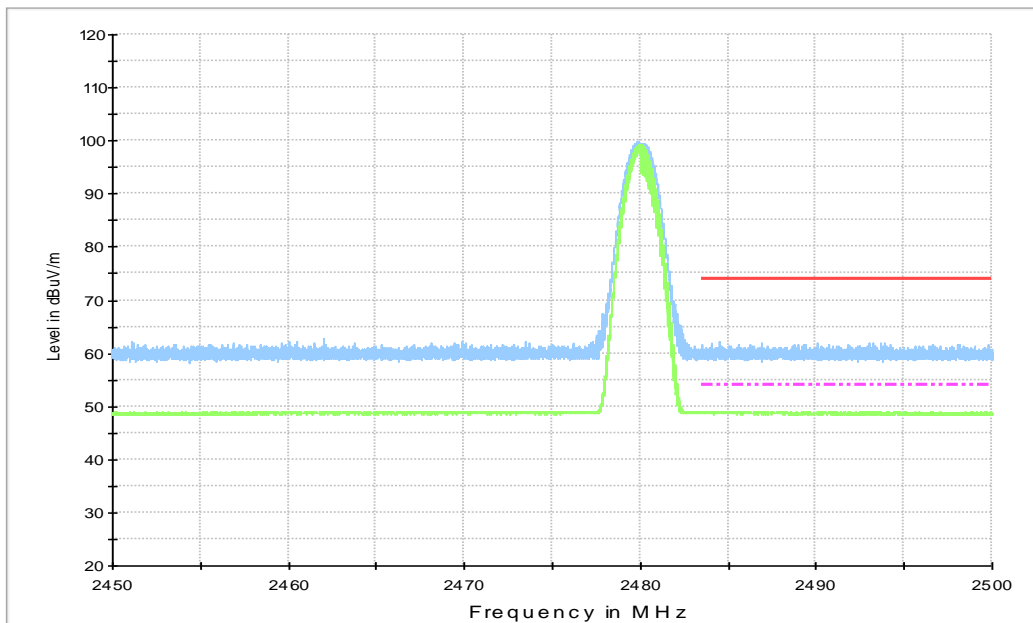
Fig.23. Frequency Band Edges: GFSK, Channel 78, 2.45 GHz - 2.50GHz
