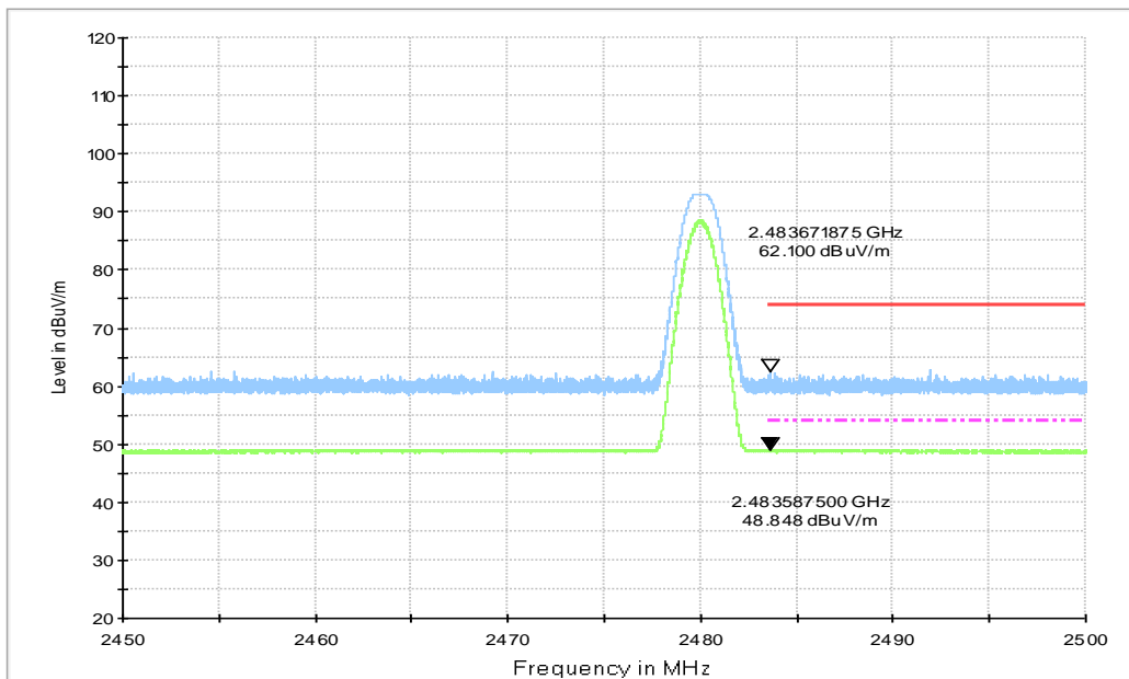
Fig.10. Frequency Band Edges: GFSK, 2480 MHz, 2.45 GHz - 2.50GHz
