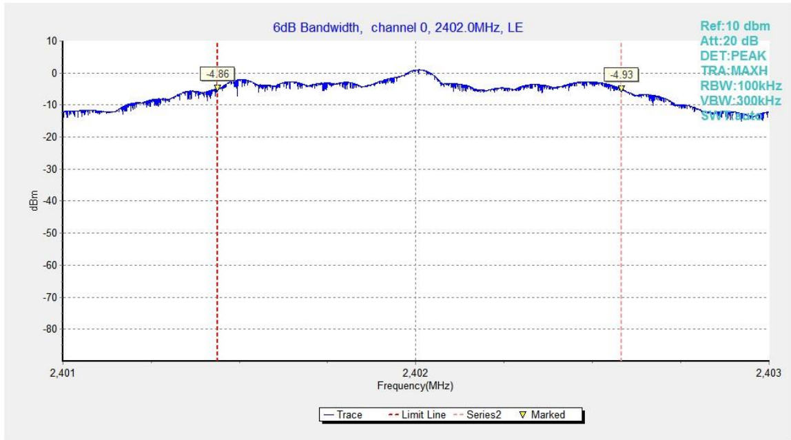
Fig.26. 6dB Bandwidth: GFSK, 2402 MHz
