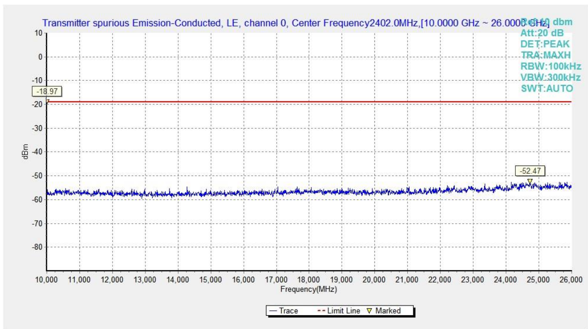
Fig.15. Transmitter Spurious Emission - Conducted: GFSK, 2402 MHz,10GHz - 26GHz
