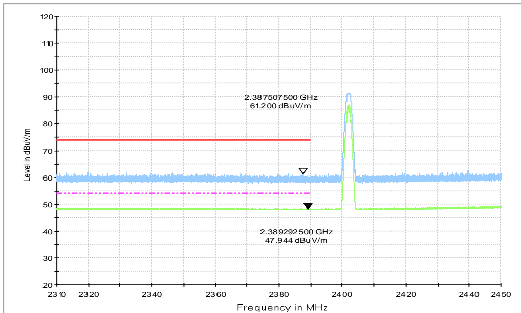
Fig.9. Frequency Band Edges: GFSK, 2402 MHz, 2.31 GHz – 2.45GHz
