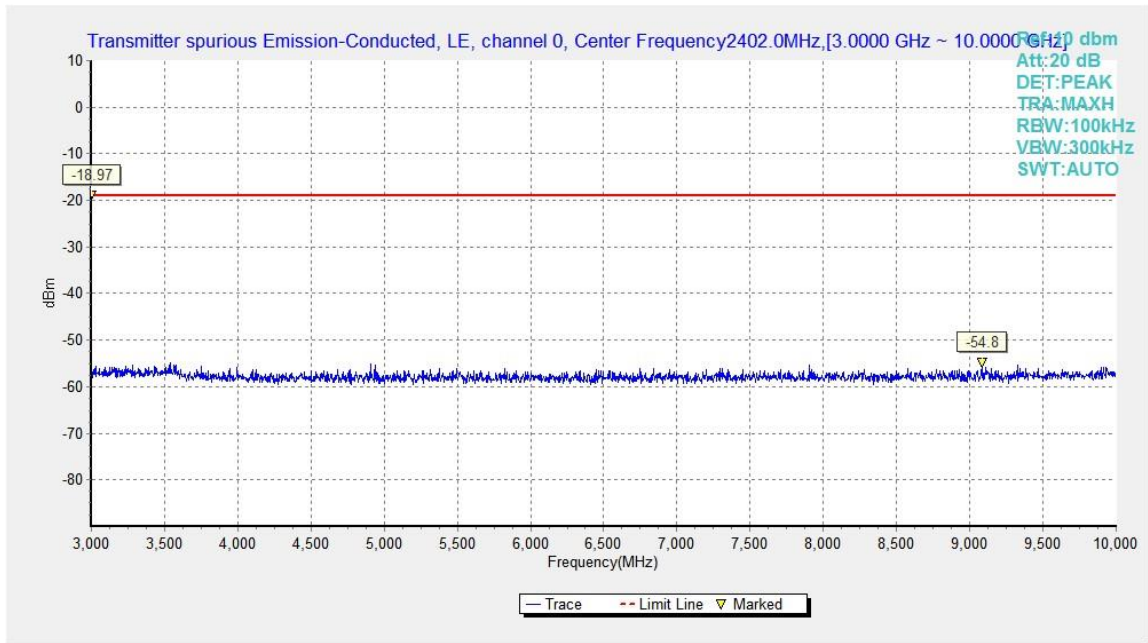
Fig.14. Transmitter Spurious Emission - Conducted: GFSK, 2402 MHz,3GHz - 10GHz
