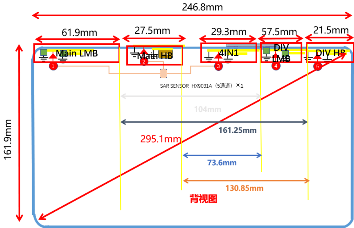
Picture 10: Antenna location
