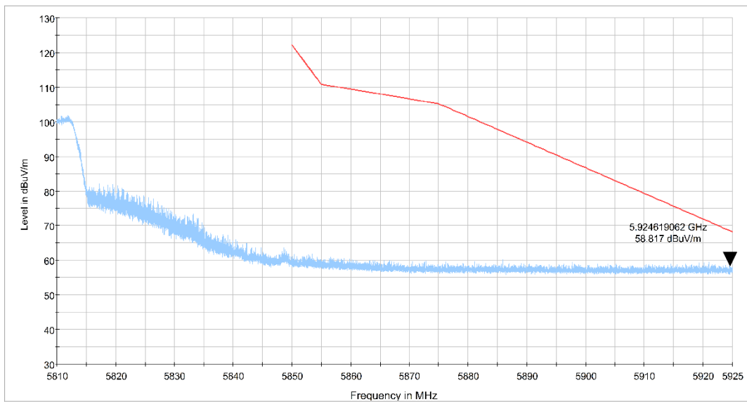
Fig. 15 Band Edges (802.11n-HT40 Ch159, 5795MHz)
