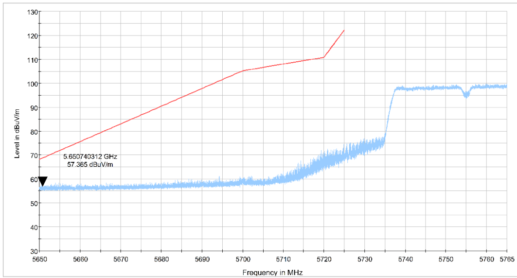
Fig. 14 Band Edges (802.11n-HT40 Ch151, 5755MHz)
