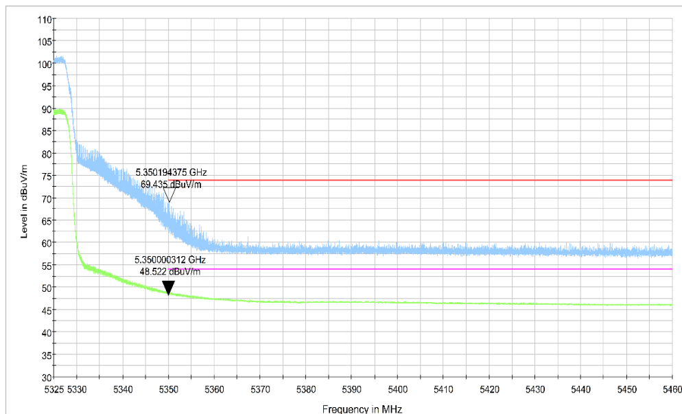
Fig.45 Band Edges (802.11n-HT40 Ch62, 5310MHz)
