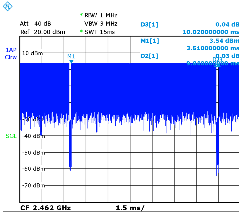
Picture 14.1-1 Duty factor plot
