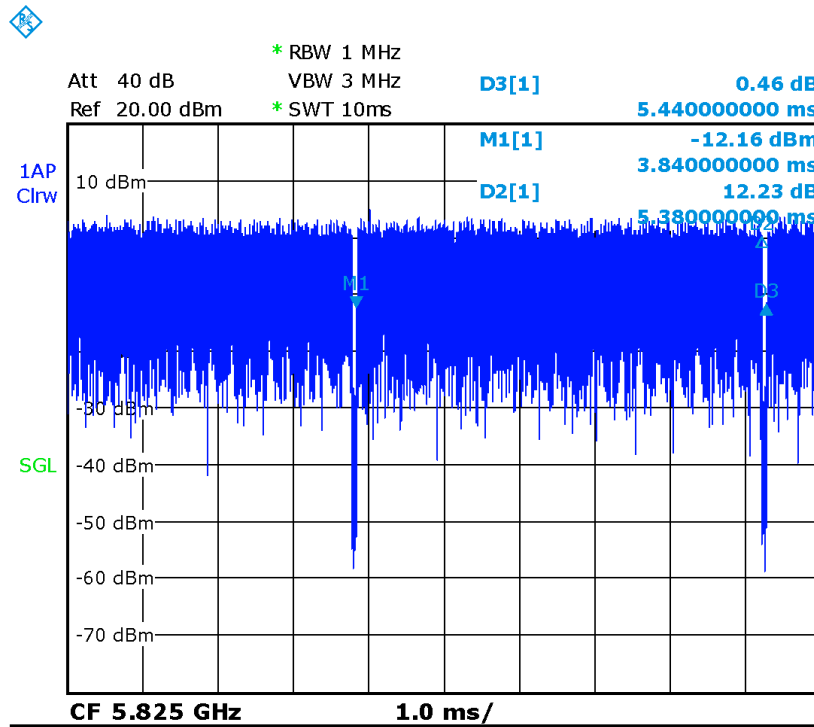
Picture 14.2-1 The plot of duty factor for CH165
