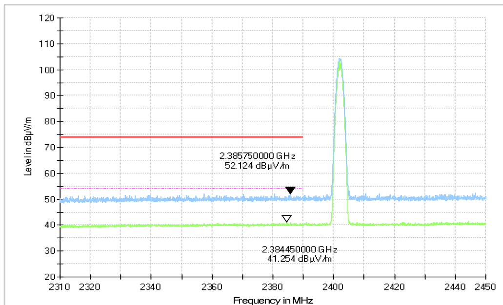
Fig.62. Frequency Band Edges: 8DPSK, Channel 0, Hopping Off, 2.31 GHz - 2.45GHz
