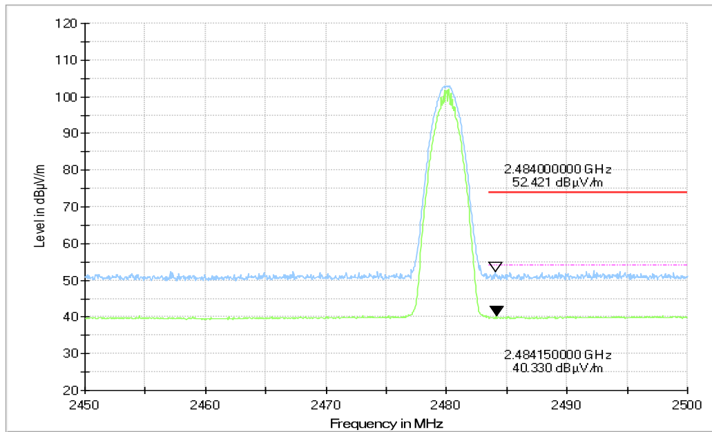
Fig.63. Frequency Band Edges: 8DPSK, Channel 78, Hopping Off, 2.45 GHz - 2.50GHz
