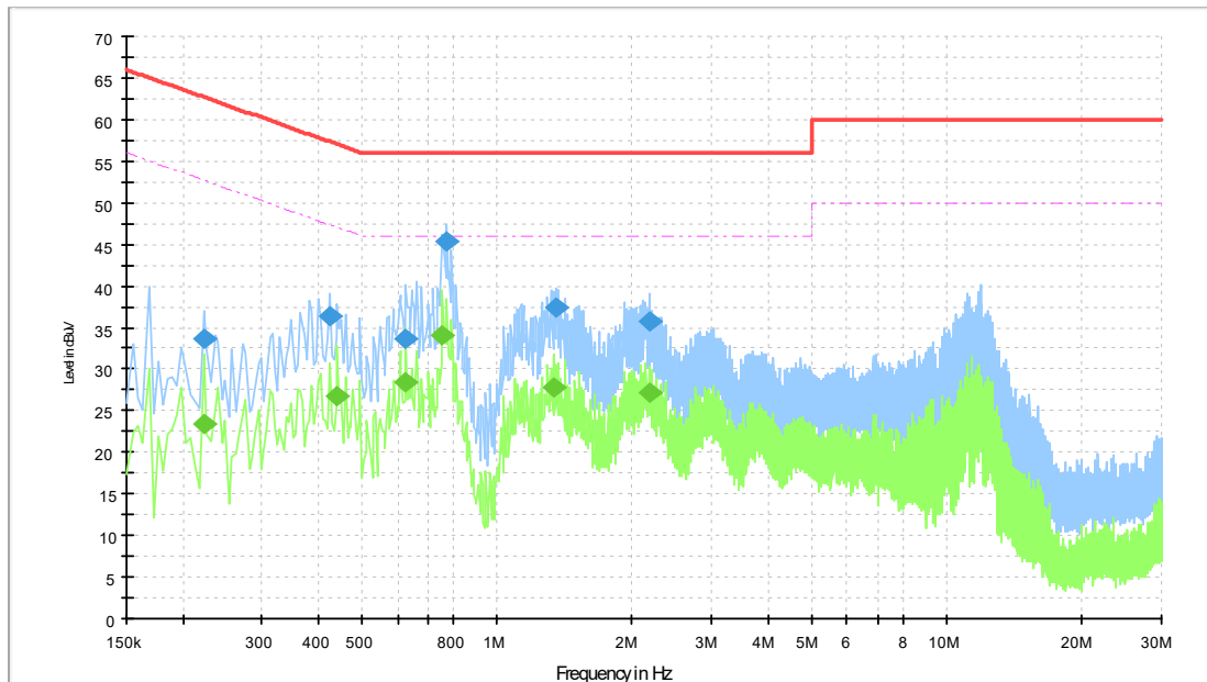
Fig.A.6.1. AC Powerline Conducted Emission-Ide
