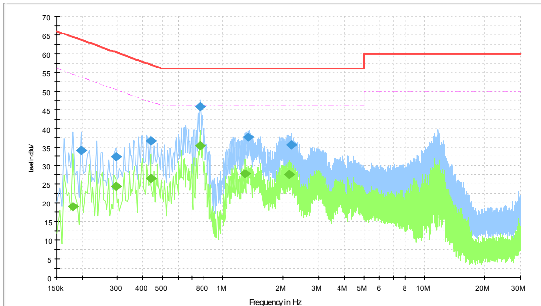
Fig.A.6.2. AC Powerline Conducted Emission-Ide
