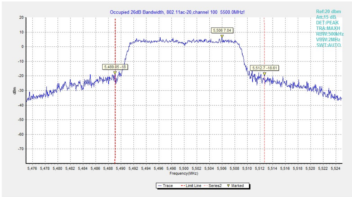
Fig.16 Occupied 26dB Bandwidth (802. 11ac-HT20, 5500MHz)
