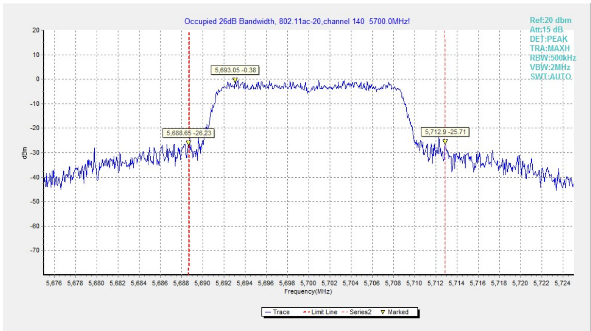
Fig.18 Occupied 26dB Bandwidth (802. 11ac-HT20, 5700MHz)
