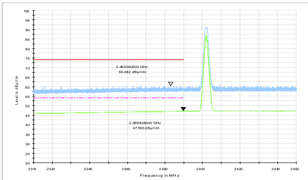
Fig.3. Frequency Band Edges: GFSK, Channel 0, 2.31GHz – 2.45GHz
