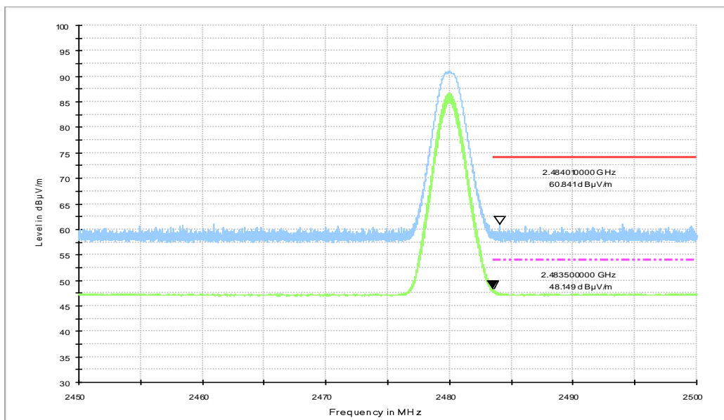
Fig.4. Frequency Band Edges: GFSK, Channel 39, 2.45GHz - 2.50GHz
