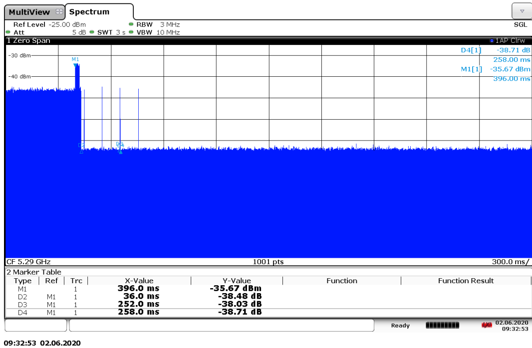
Fig.A.3 channel closing transmission time
