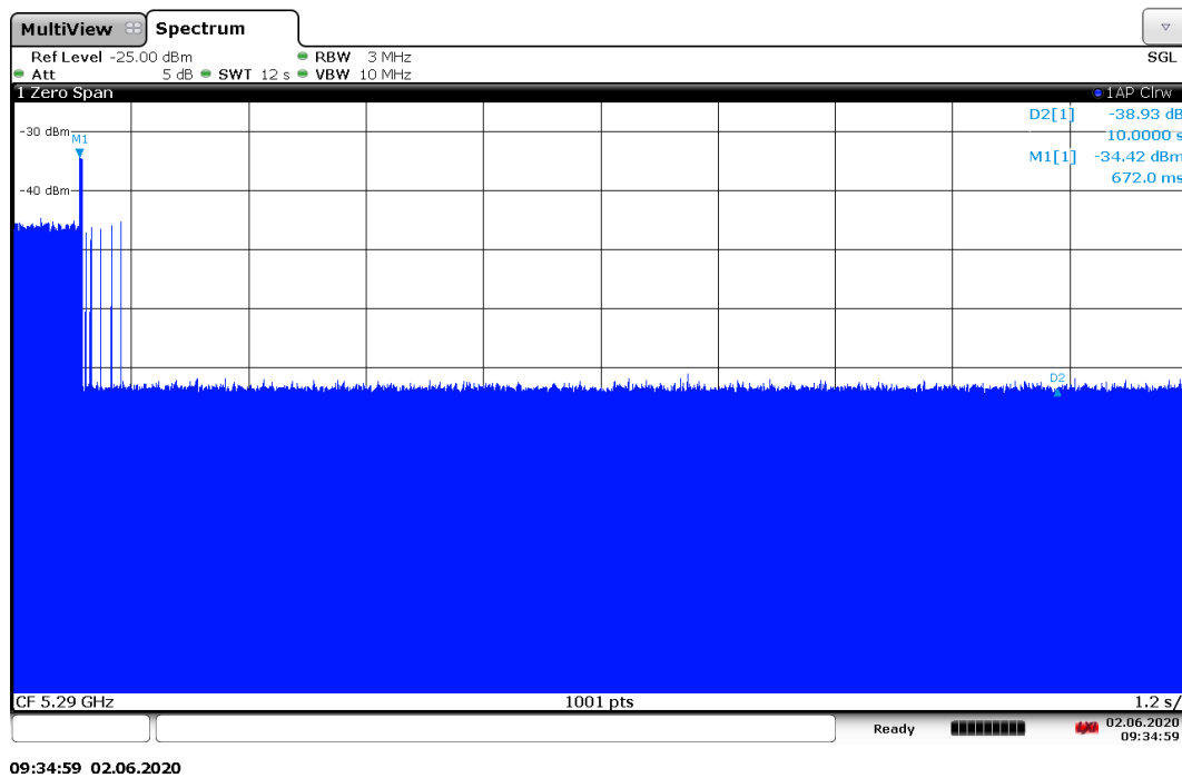
Fig.A.2 Channel move time
