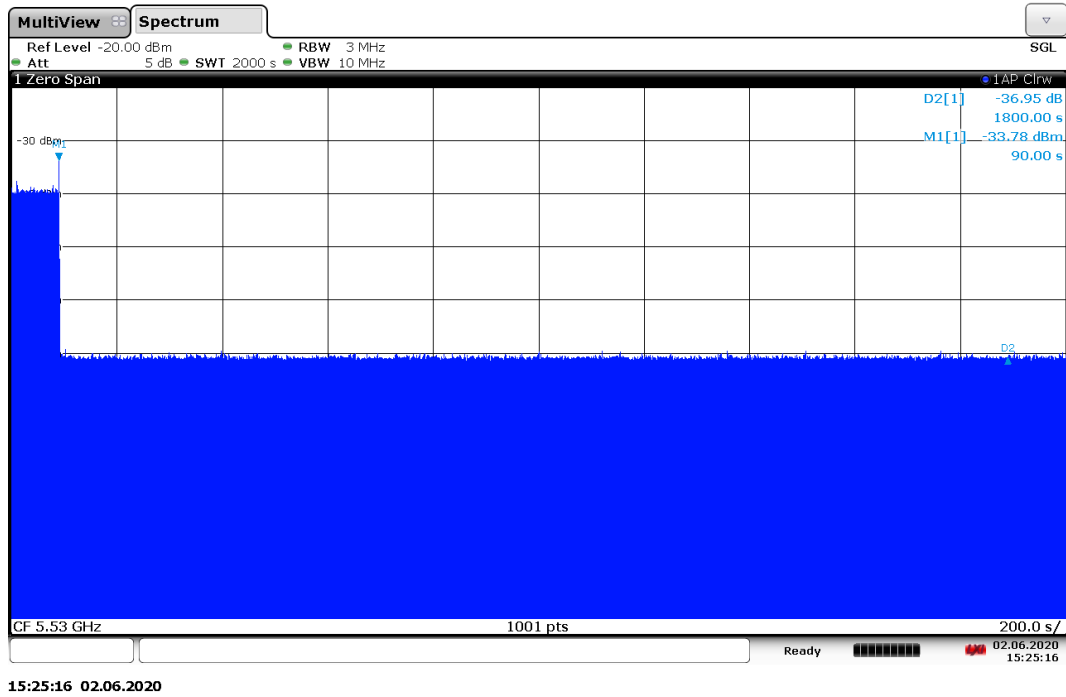
Fig.A.7 Non-Occupancy Period
