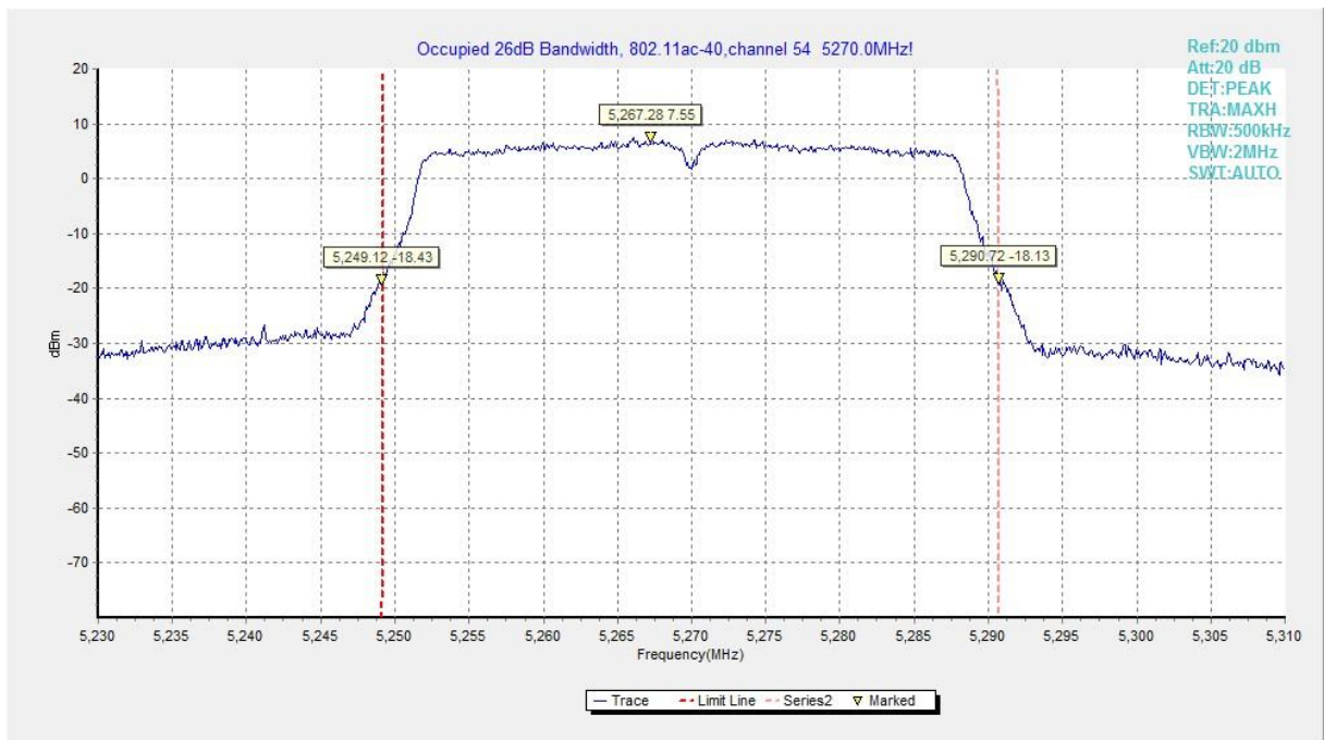
Fig.40 Occupied 26dB Bandwidth (802.11ac-HT40, 5270MHz)
