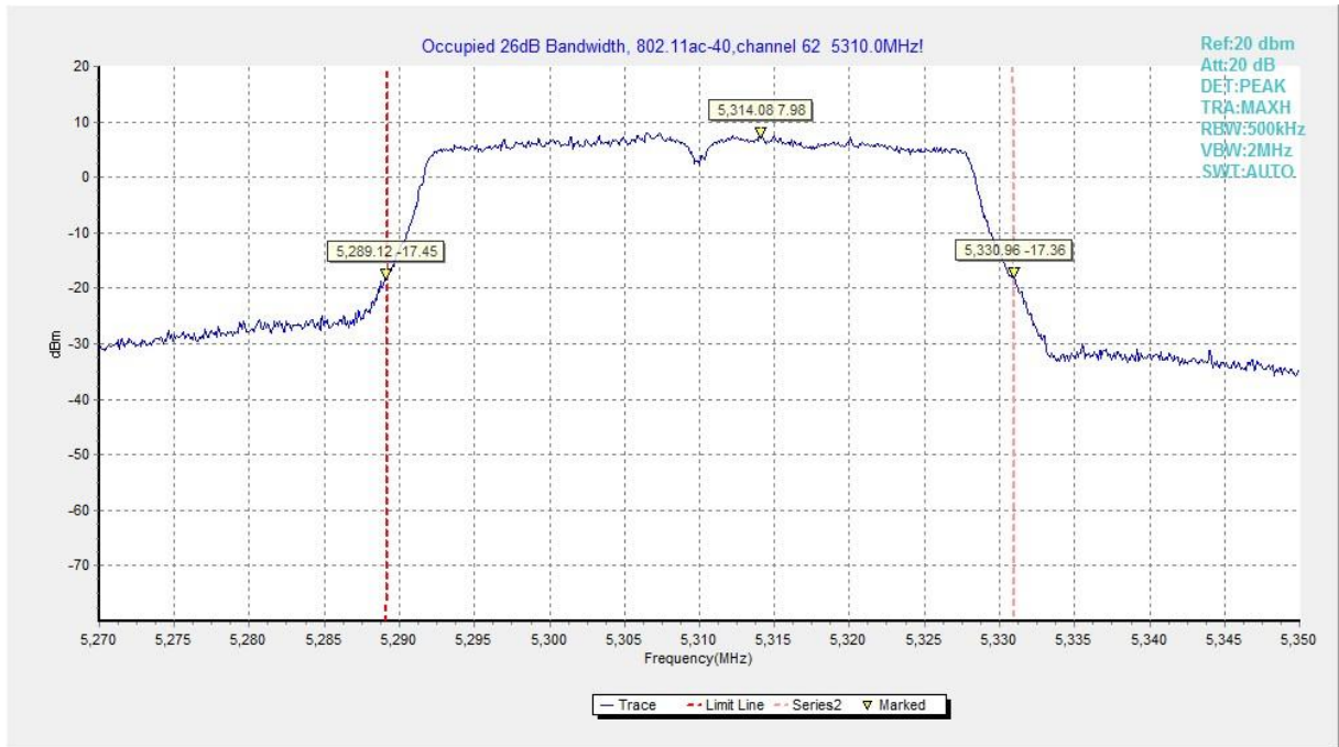
Fig.41 Occupied 26dB Bandwidth (802.11ac-HT40, 5310MHz)
