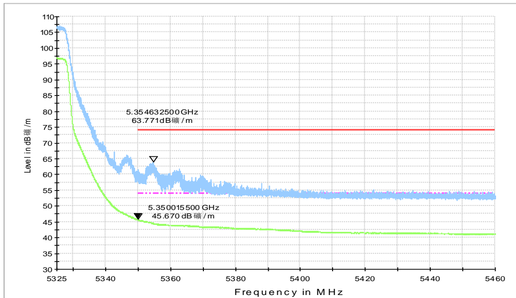
Fig.50 Band Edges (802.11a, 5320MHz)
