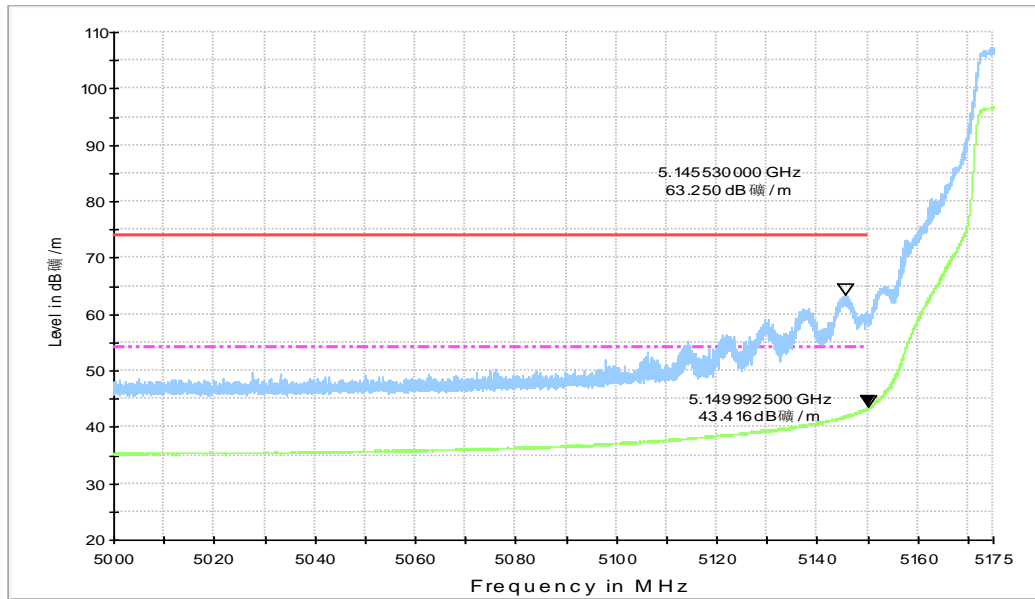
Fig.49 Band Edges (802.11a, 5180MHz)
