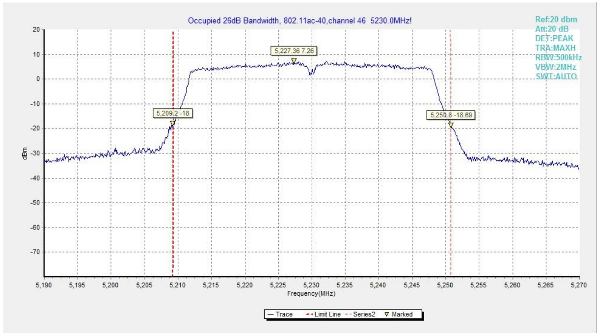
Fig.39 Occupied 26dB Bandwidth (802.11ac-HT40, 5230MHz)
