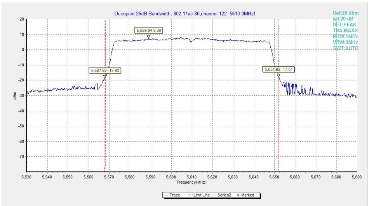
Fig.48 Occupied 26dB Bandwidth (802.11ac-HT80, 5610MHz)
