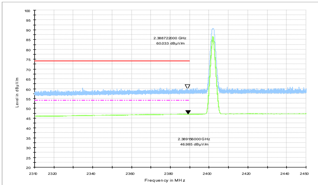
Fig.3. Frequency Band Edges: GFSK, Channel 0, 2.31GHz – 2.45GHz
