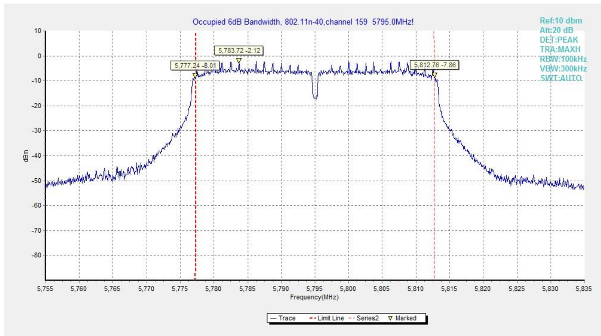
Fig. 8 Occupied 6dB Bandwidth (802.11n40, Ch 159)
