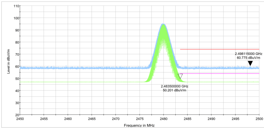
Fig.14. Frequency Band Edges: GFSK, Channel 78, 2.45 GHz - 2.50GHz
