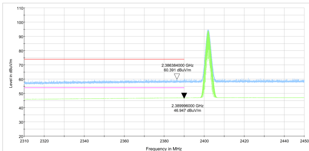
Fig.13. Frequency Band Edges: GFSK, Channel 0, 2.31 GHz – 2.45GHz
