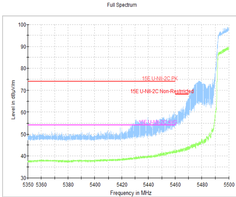
Fig.44 Band Edges (802.11n-HT40, 5510MHz)
