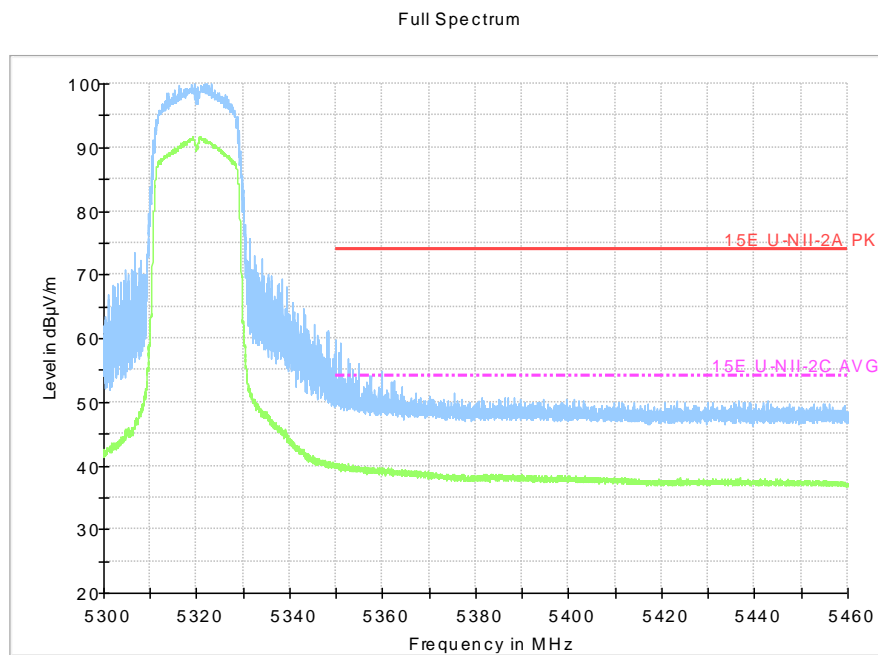
Fig.35 Band Edges (802.11n-HT20, 5320MHz)
