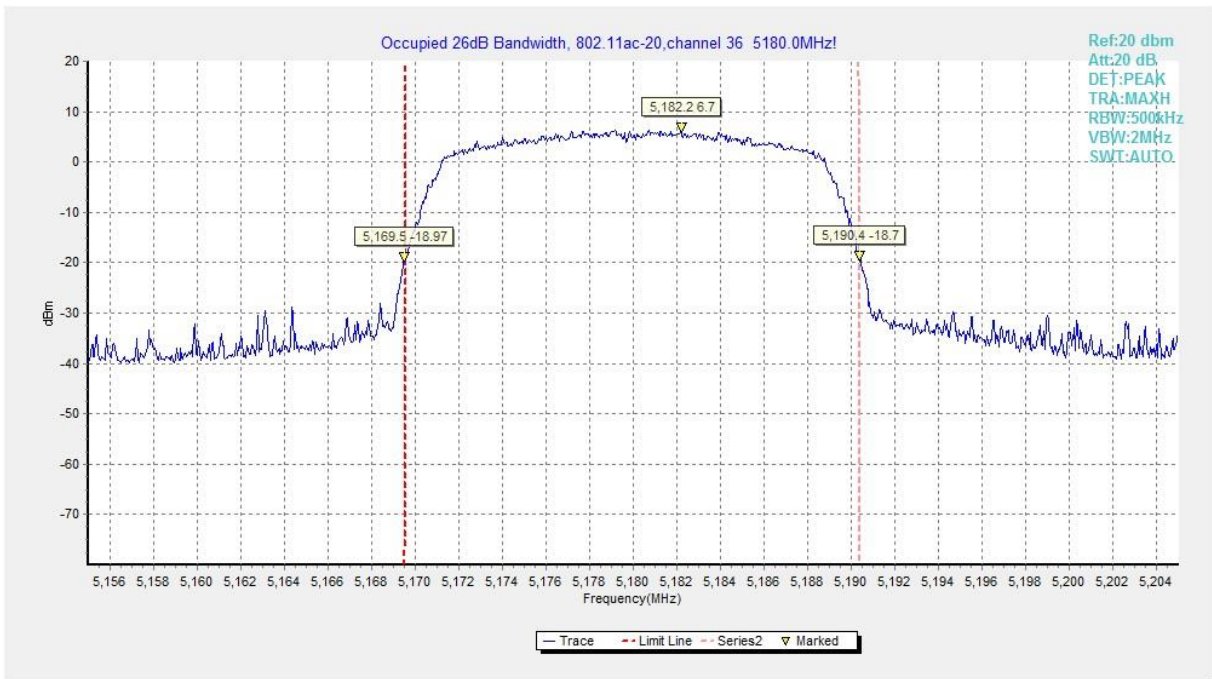
Fig.10 Occupied 26dB Bandwidth (802.11ac-HT20, 5180MHz)
