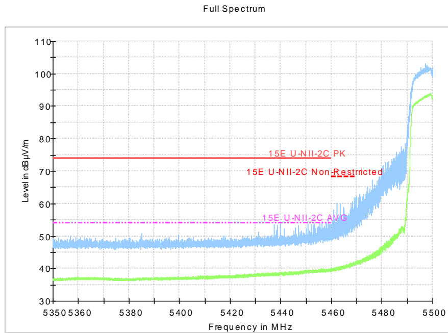
Fig.32 Band Edges (802.11a, 5500MHz)
