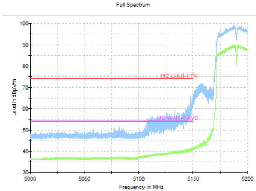
Fig.38 Band Edges (802.11n-HT40, 5190MHz)
