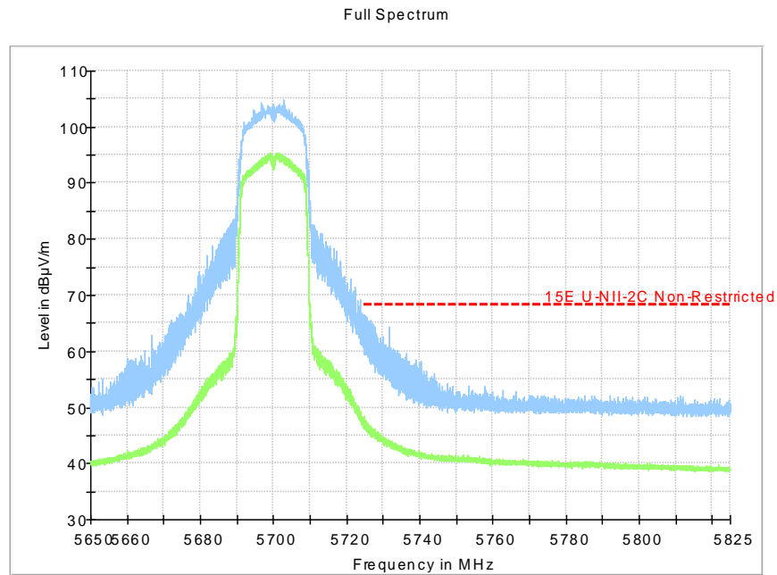
Fig.37 Band Edges (802.11n-HT20, 5700MHz)
