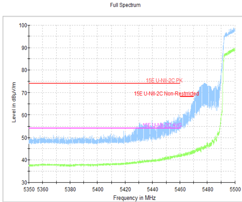
Fig.40 Band Edges (802.11n-HT40, 5510MHz)
