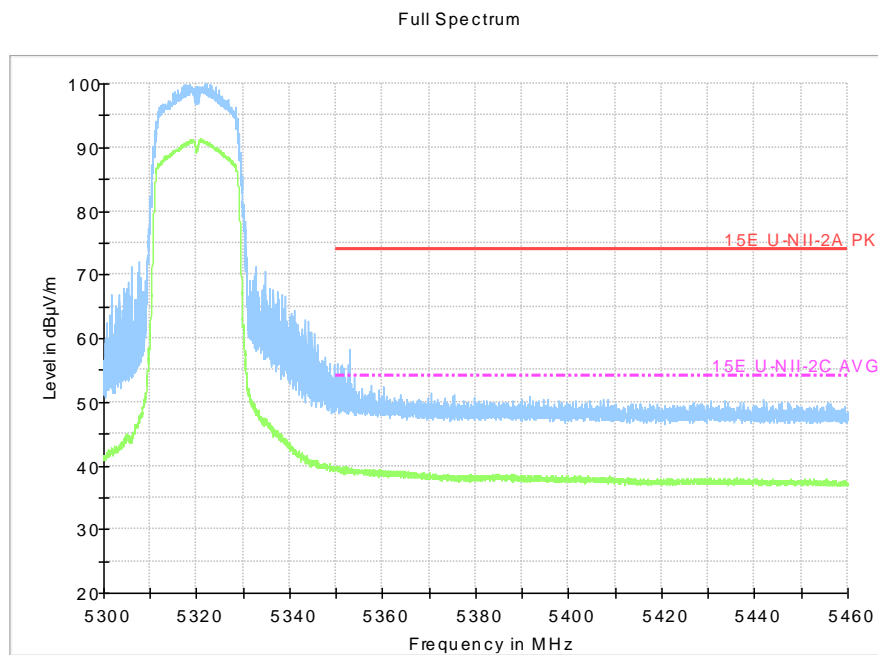
Fig.43 Band Edges (802.11ac-HT20, 5320MHz)
