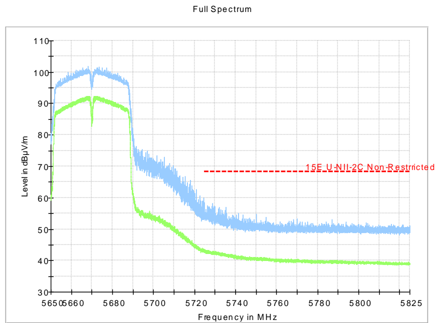
Fig.49 Band Edges (802.11ac-HT40, 5670MHz)
