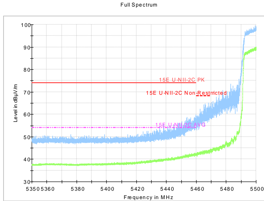
Fig.48 Band Edges (802.11ac-HT40, 5510MHz)
