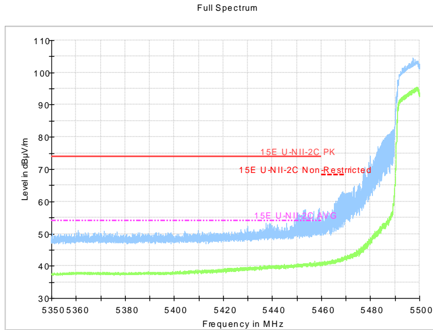
Fig.36 Band Edges (802.11n-HT20, 5500MHz)
