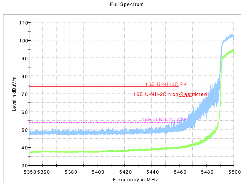
Fig.44 Band Edges (802.11ac-HT20, 5500MHz)
