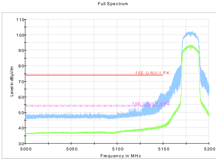
Fig.34 Band Edges (802.11n-HT20, 5180MHz)
