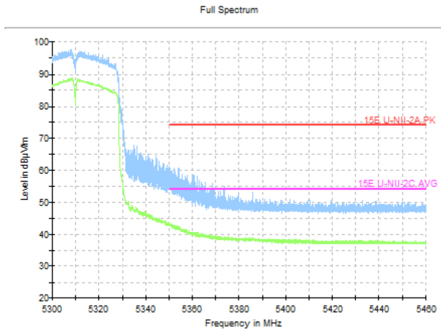
Fig.39 Band Edges (802.11n-HT40, 5310MHz)
