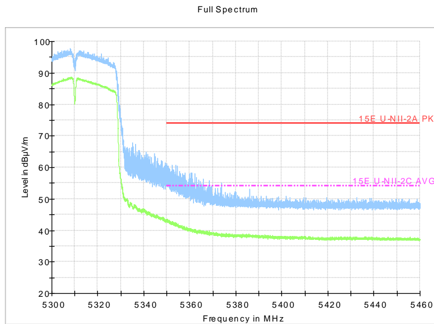
Fig.47 Band Edges (802.11ac-HT40, 5310MHz)
