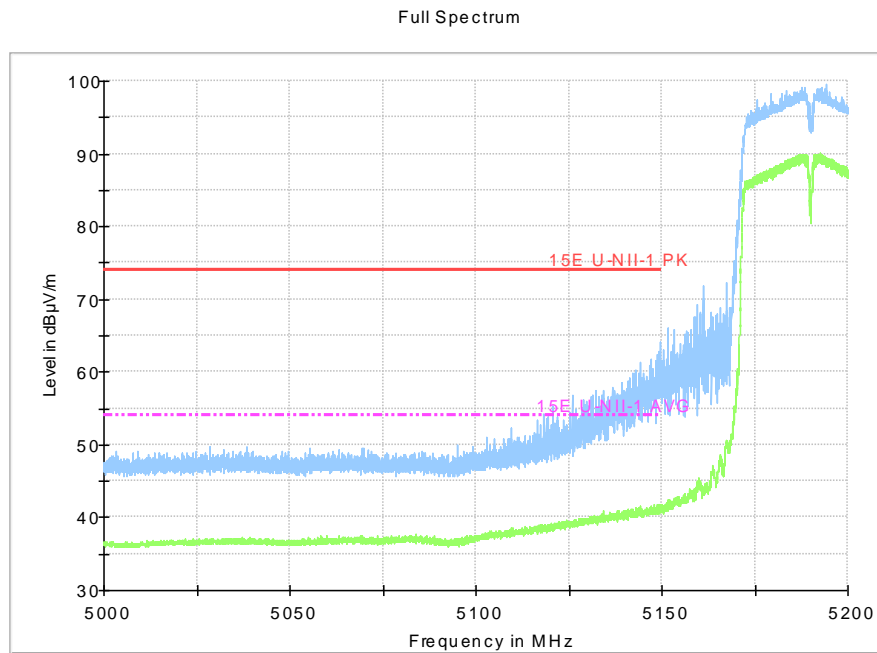
Fig.46 Band Edges (802.11ac-HT40, 5190MHz)
