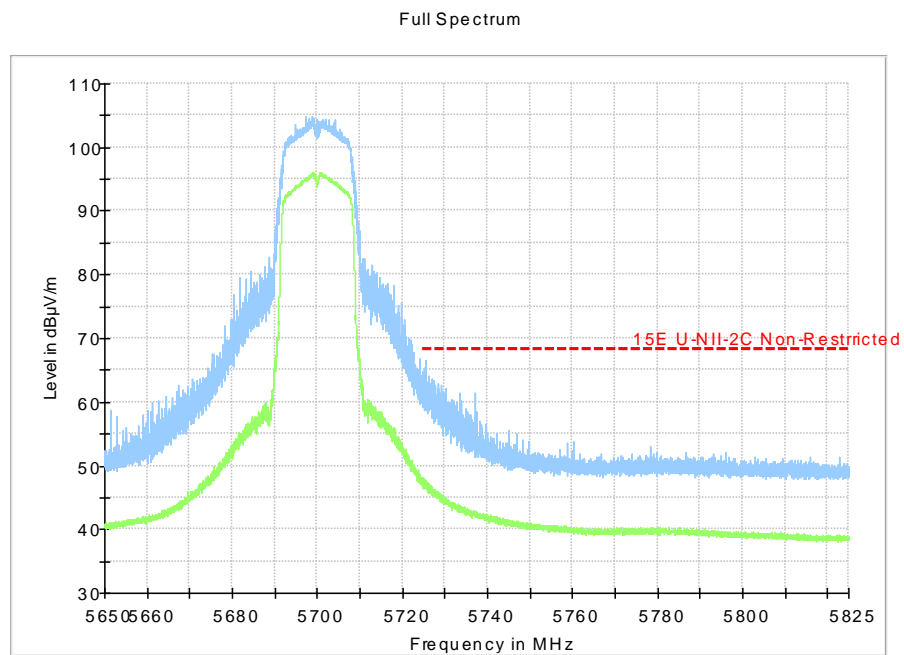
Fig.33 Band Edges (802.11a, 5700MHz)
