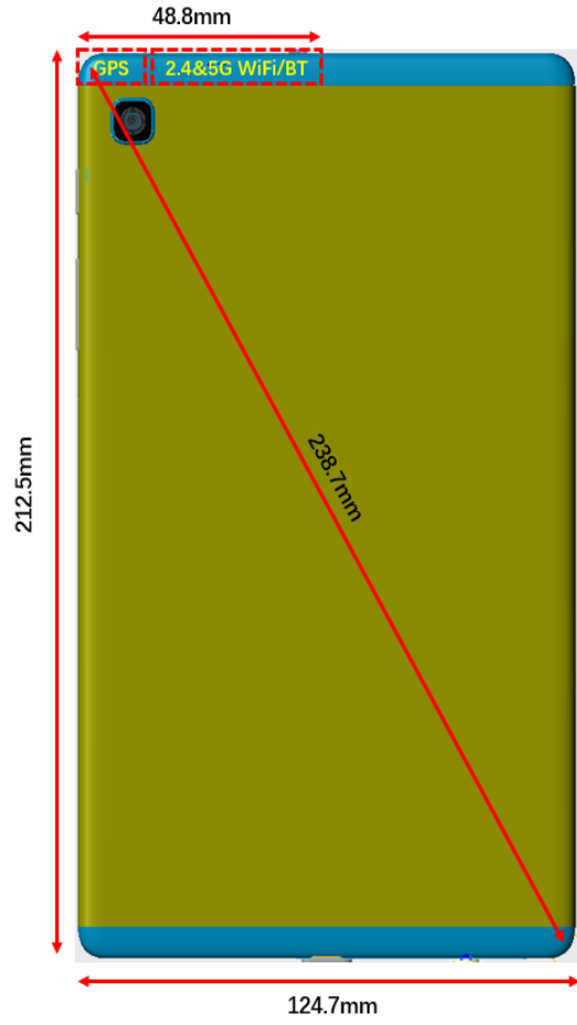
Picture 9 Antenna Locations
