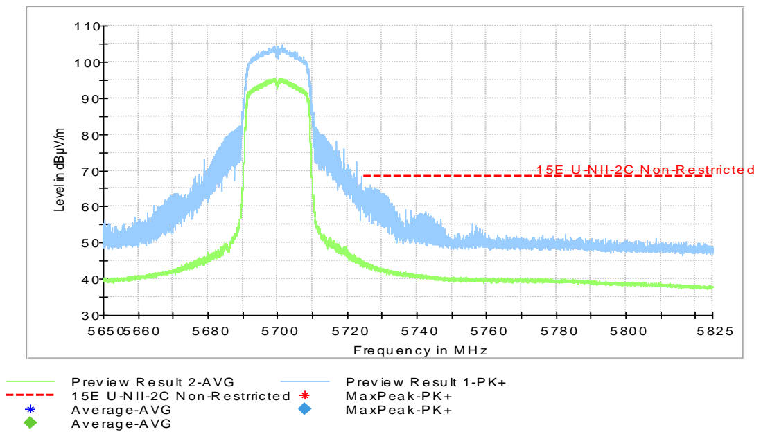
Fig.41 Band Edges (802.11n-HT20, 5700MHz)
