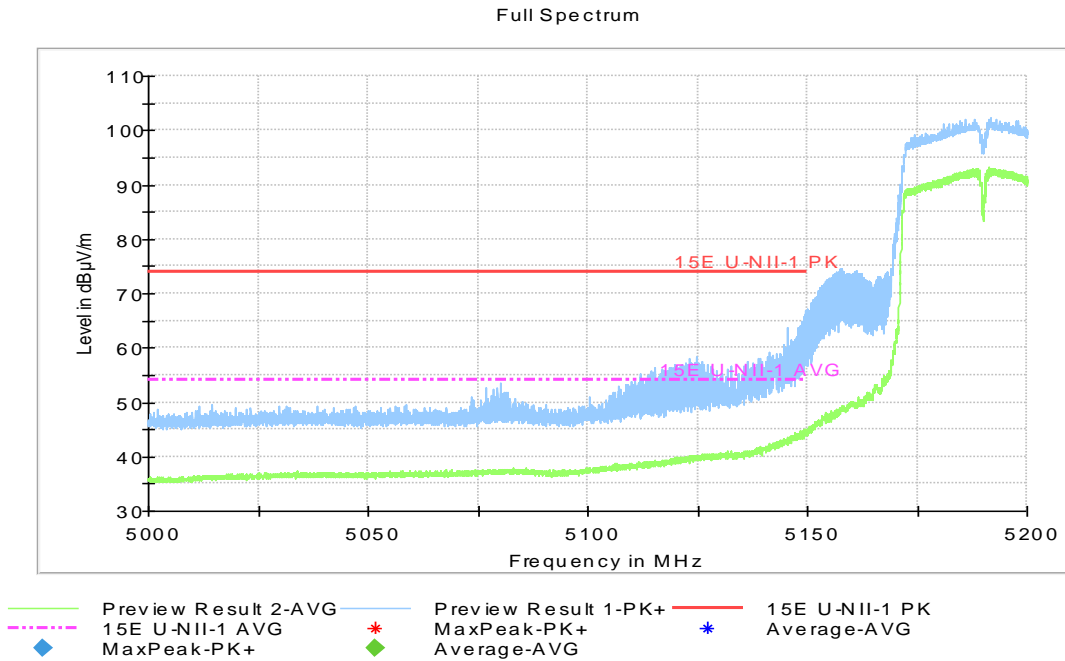
Fig.42 Band Edges (802.11n-HT40, 5190MHz)
