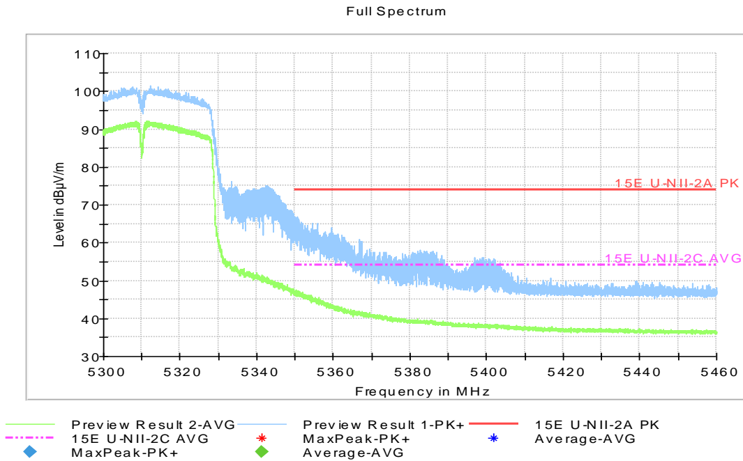
Fig.43 Band Edges (802.11n-HT40, 5310MHz)
