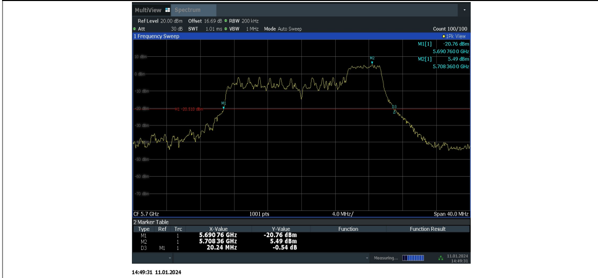
11AX20SISO_Ant6_5700_106Tone_RU54
