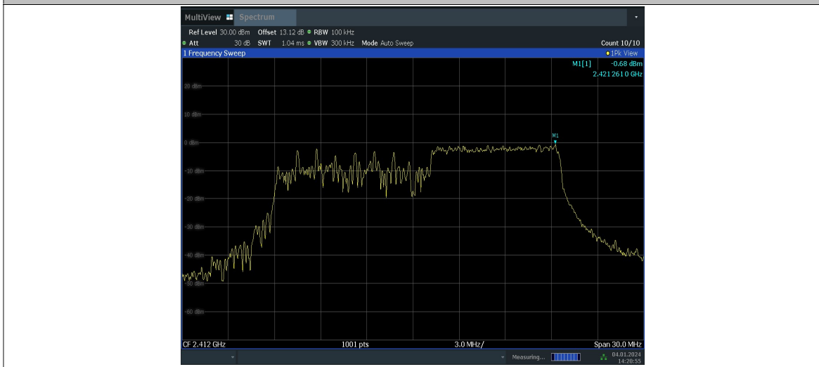
11AX20SISO_Ant10_2412_106Tone_RU54_0~Reference
