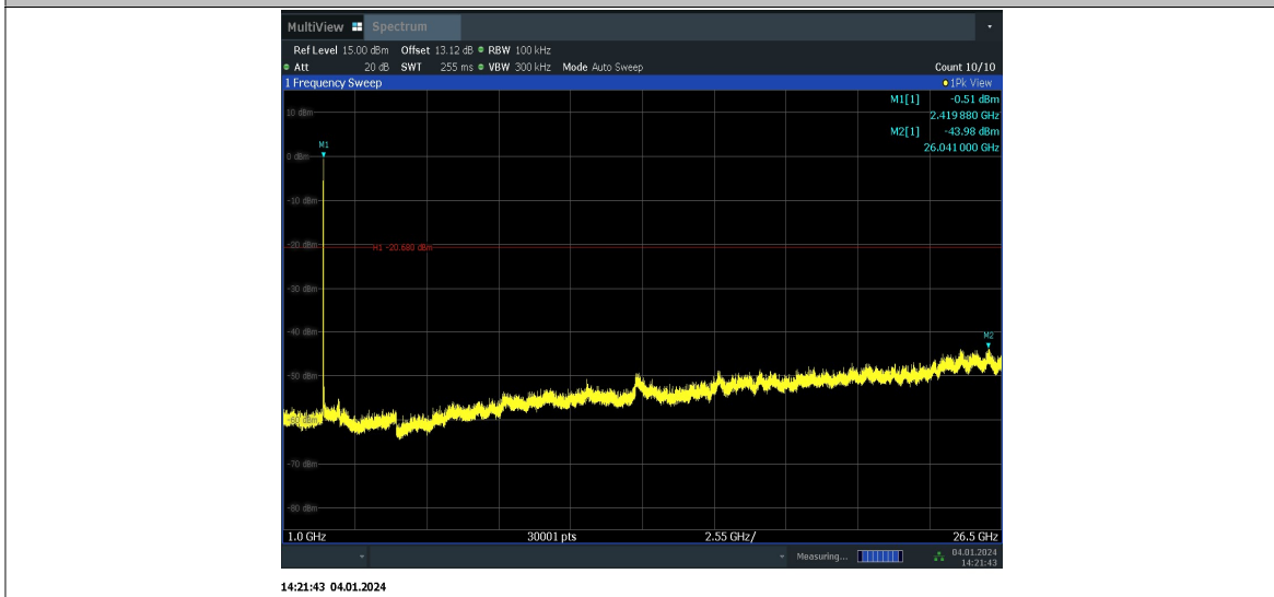
11AX20SISO_Ant10_2437_26Tone_RU0_0~Reference
