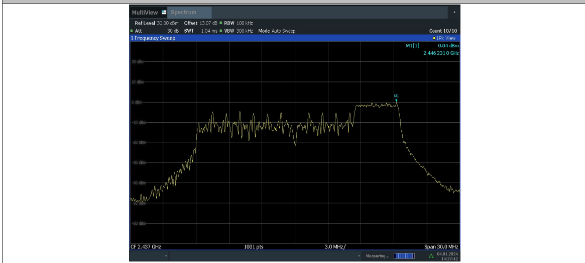
11AX20SISO_Ant10_2437_52Tone_RU40_0~Reference
