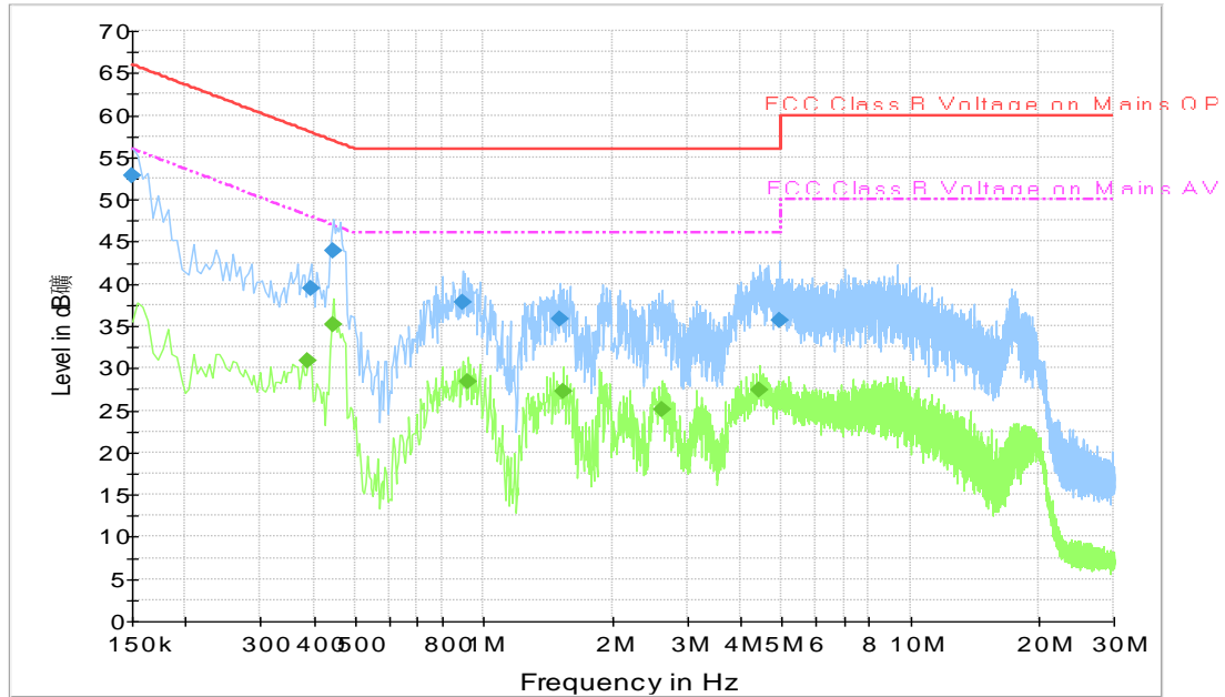
Fig.A.7.3 AC Powerline Conducted Emission-802.11b
