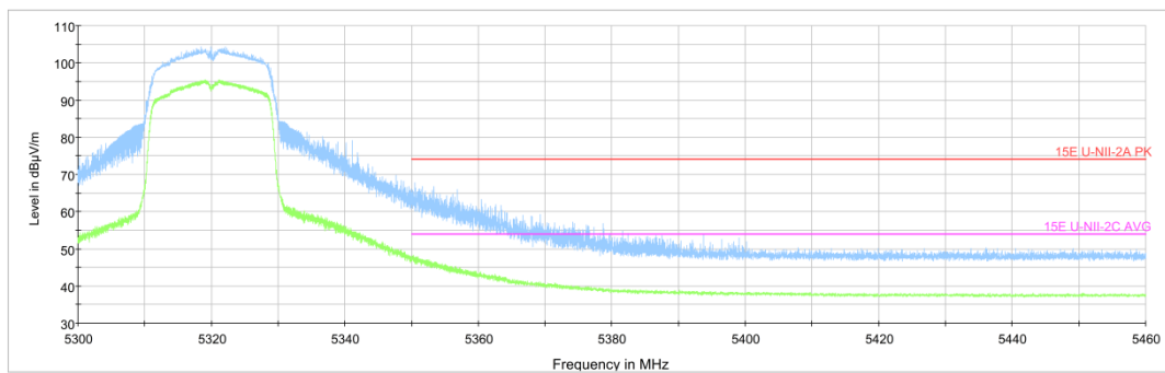
Fig.35 Band Edges (802.11n-HT20 Ch64, 5320MHz)
