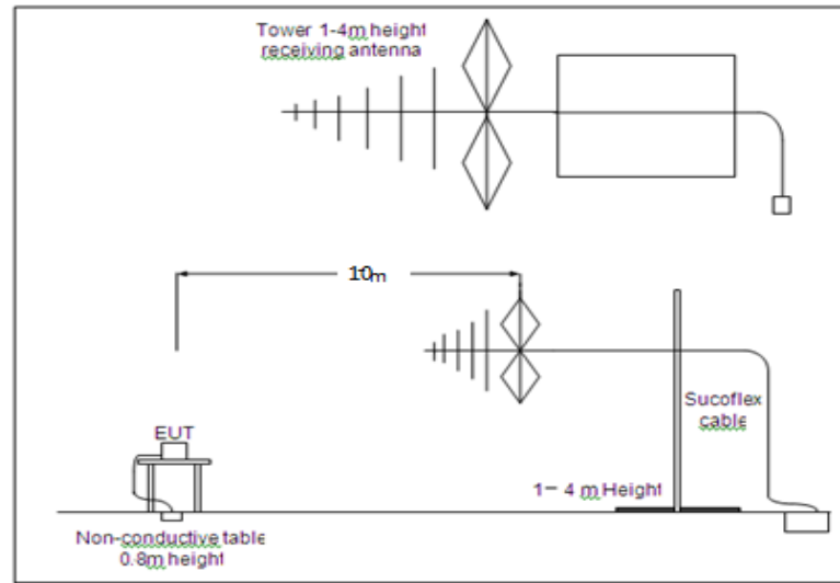
Figure B-5: Measurement Setup
