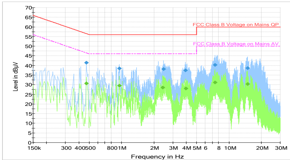
Figure B-11: Measurement results for Conducted Emission
