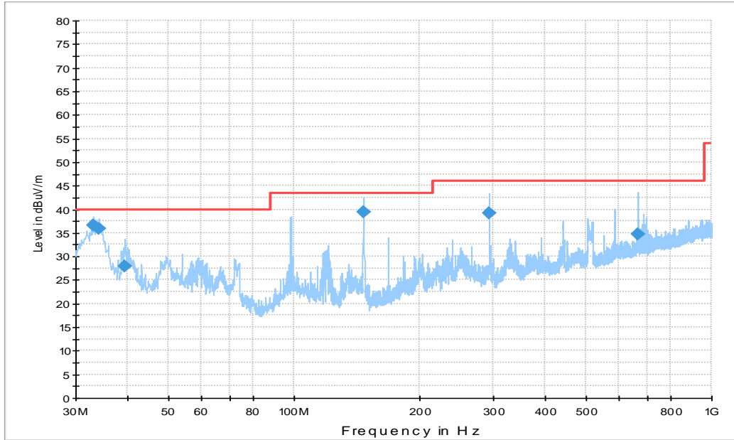
Figure A.8 Radiated Emission from 30MHz to 1GHz
