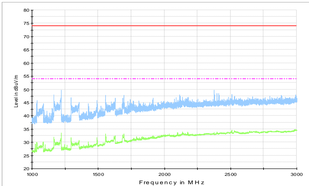
Figure A.9 Radiated Emission from 1GHz to 3GHz
