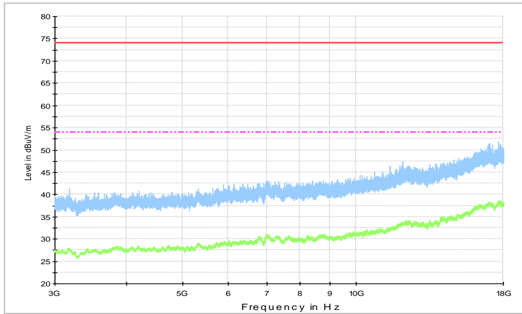
Figure A.7 Radiated Emission from 3GHz to 18GHz
