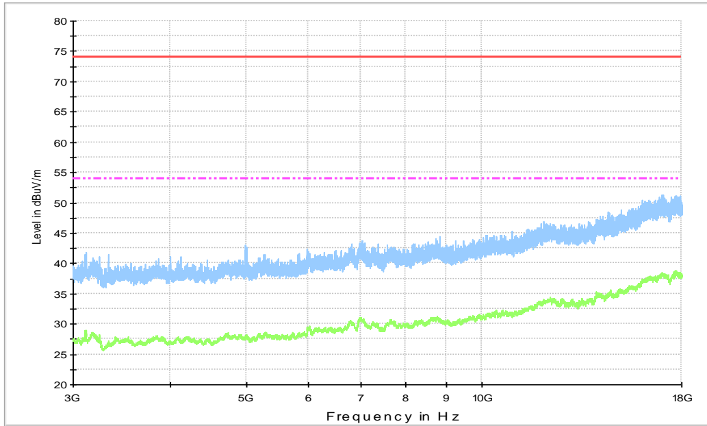
Figure A.10 Radiated Emission from 3GHz to 18GHz
