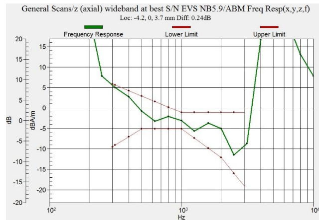
Figure C.7 Frequency Response of WCDMA 1900 - OTT VoIP
