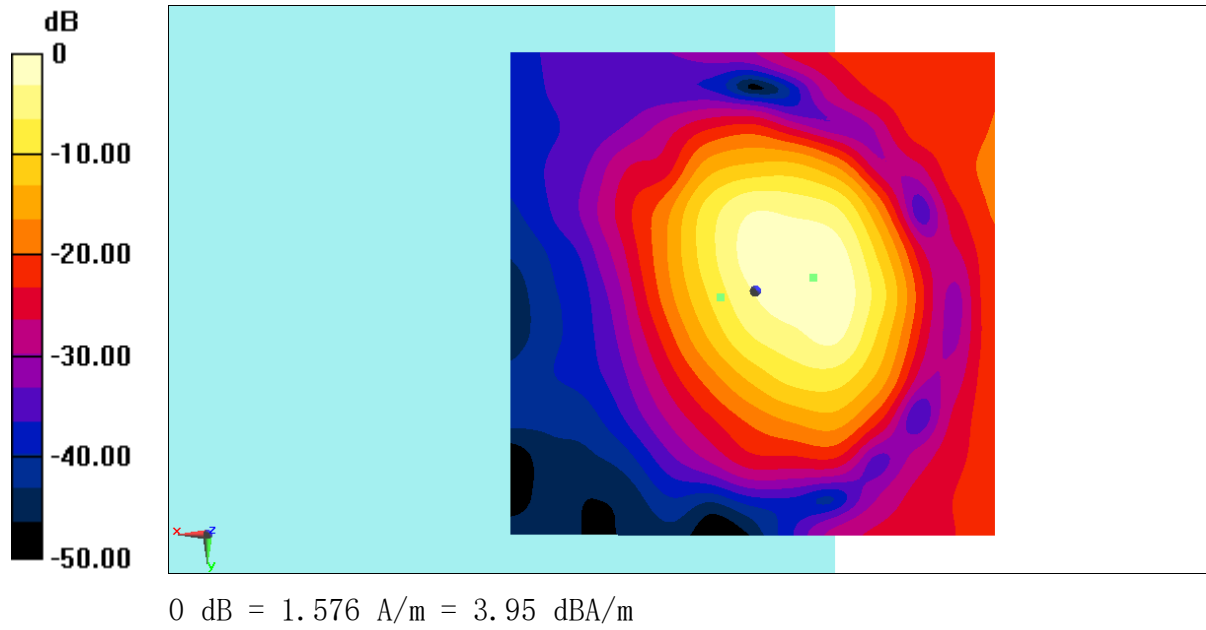
Fig B.18 T-Coil LTE B41
