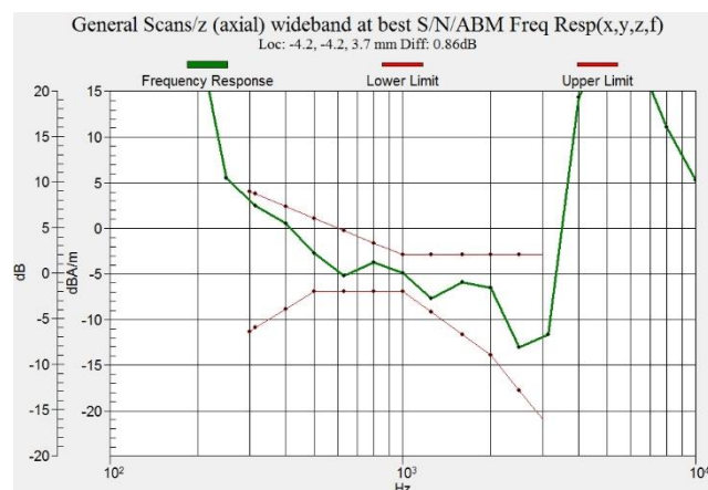
Figure C.9 Frequency Response of LTE B41 PC3 - OTT VoIP
