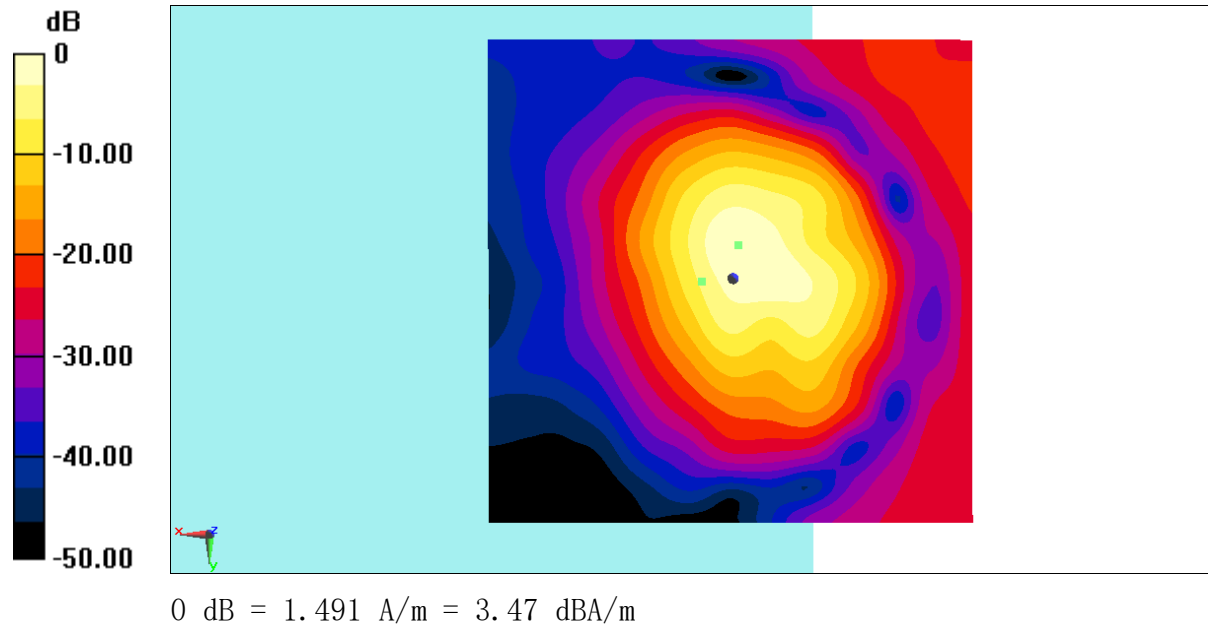
Fig B.18 T-Coil LTE B7
