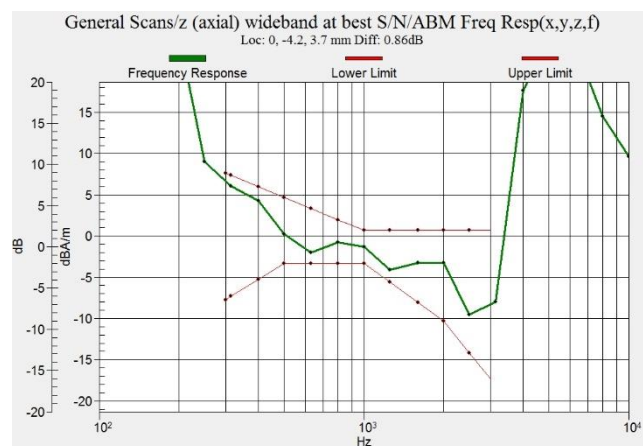
Figure C.9 Frequency Response of LTE B7 - OTT VoIP
