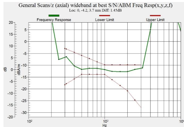
Figure C.4 Frequency Response of LTE B12
