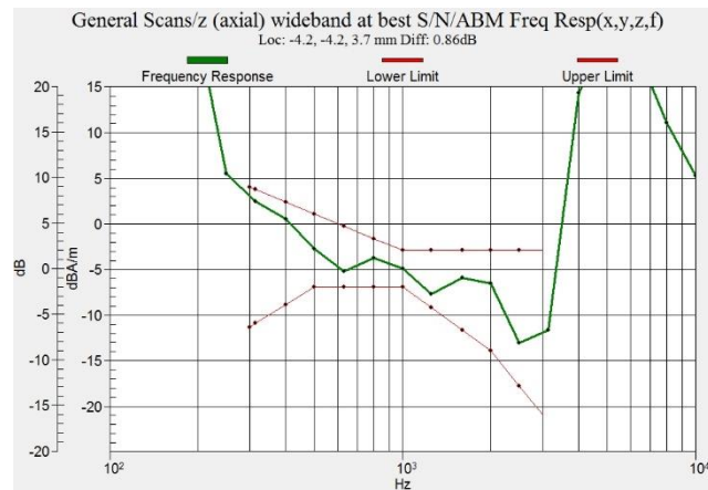
Figure C.10 Frequency Response of LTE B41 PC3 - OTT VoIP
