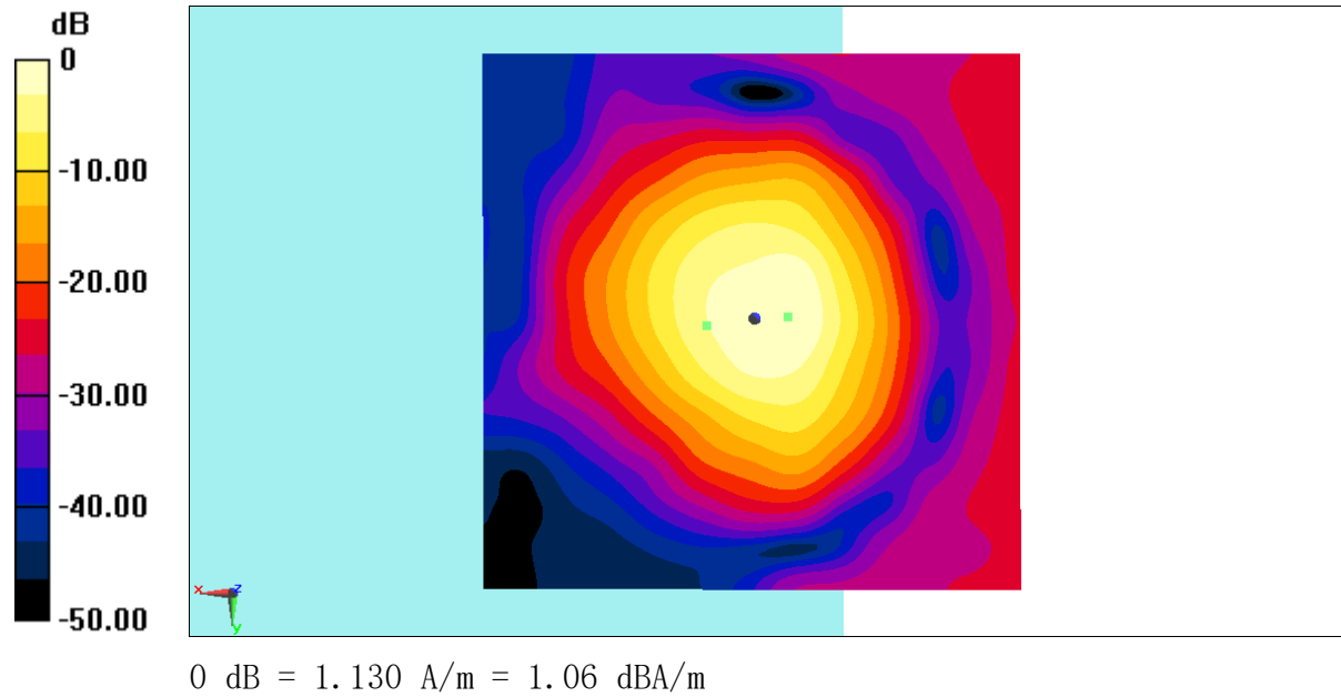
Fig B.16 T-Coil CDMA BC1
