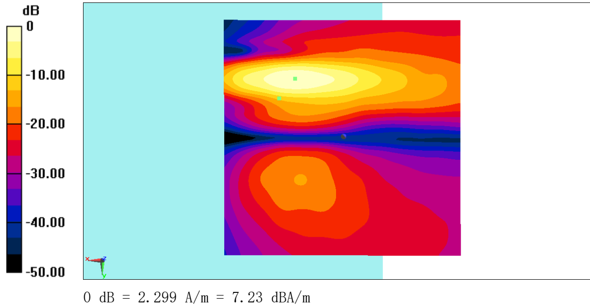
Fig B.9 T-Coil LTE B41
