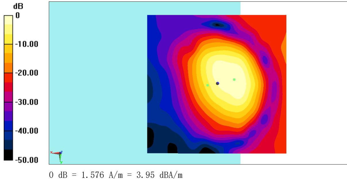
Fig B.20 T-Coil LTE B41
