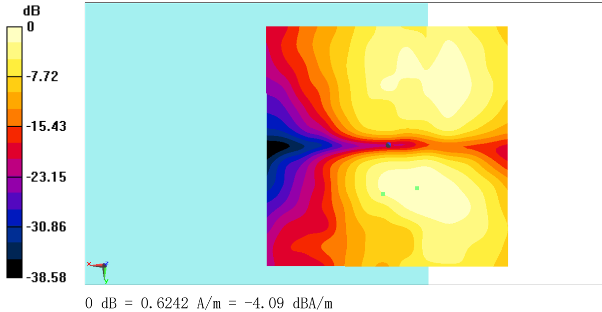
Fig B.17 T-Coil LTE B7
