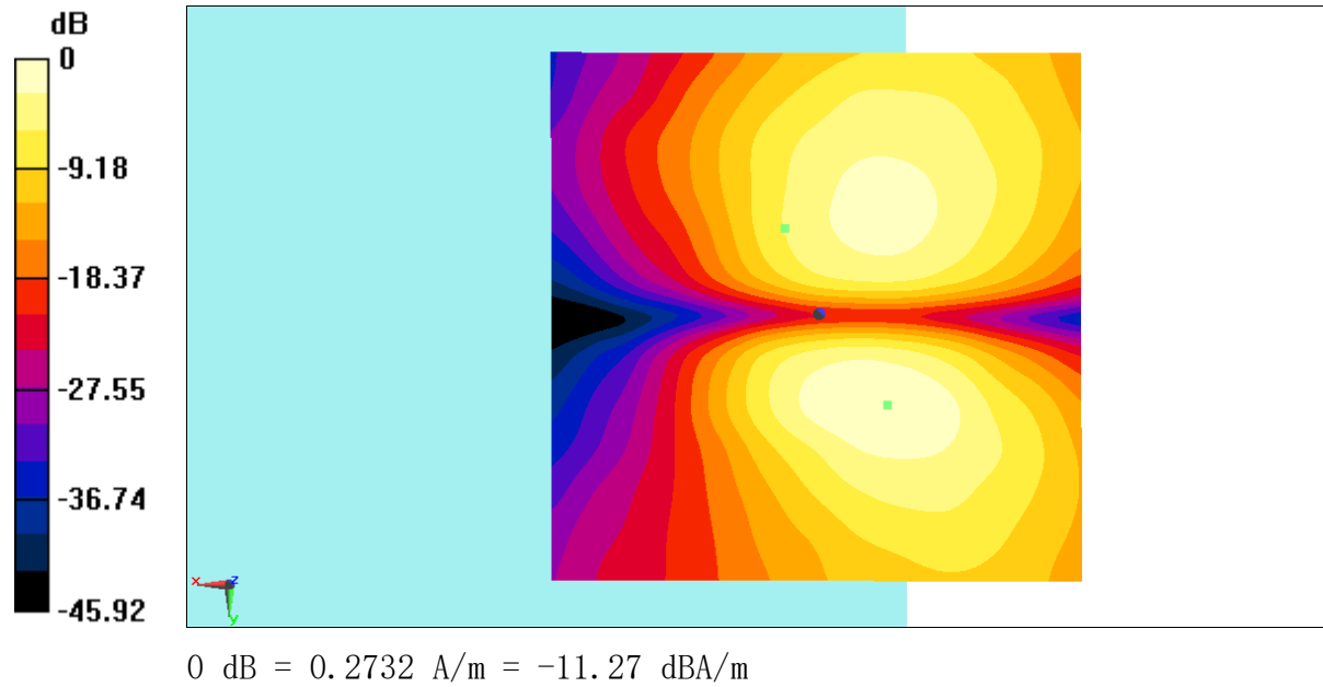
Fig B.7 T-Coil LTE B7
