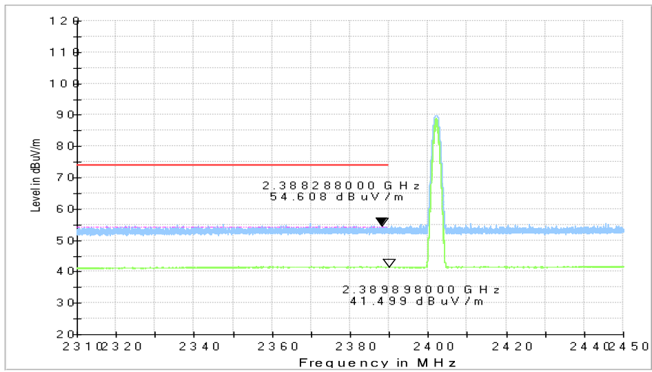
Fig.3. Frequency Band Edges: GFSK, 2402 MHz, 2.31 GHz – 2.45GHz
