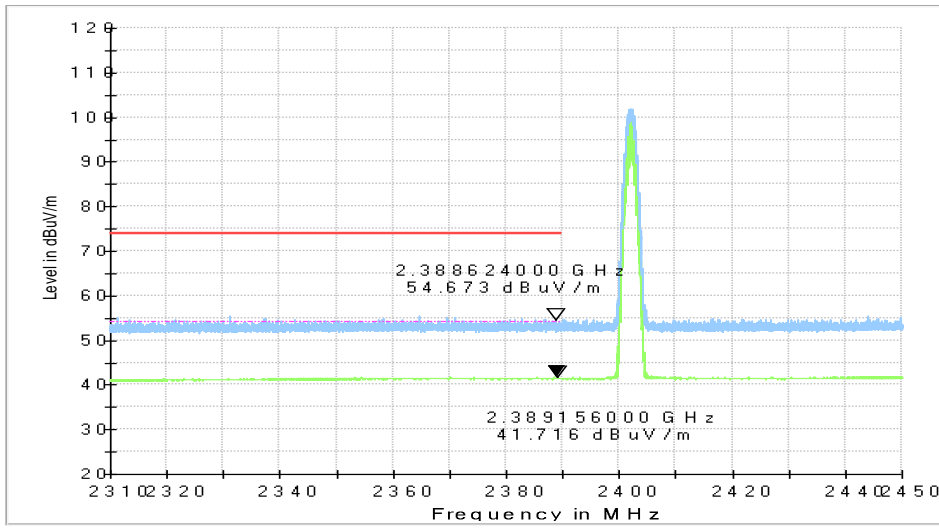
Fig.13. Frequency Band Edges: GFSK, Channel 0, 2.31 GHz – 2.45GHz
