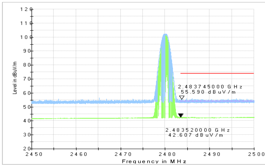
Fig.14. Frequency Band Edges: GFSK, Channel 78, 2.45 GHz - 2.50GHz
